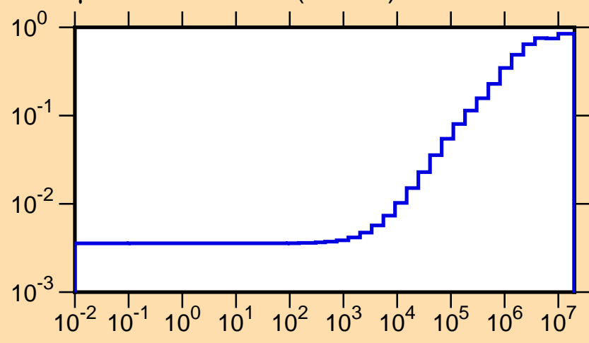
\mu vs. E for ^{193}\text{Os}(\text{mt251})
