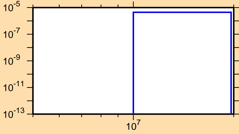
\sigma vs. E for ^{193}\text{Os}(n,t)
