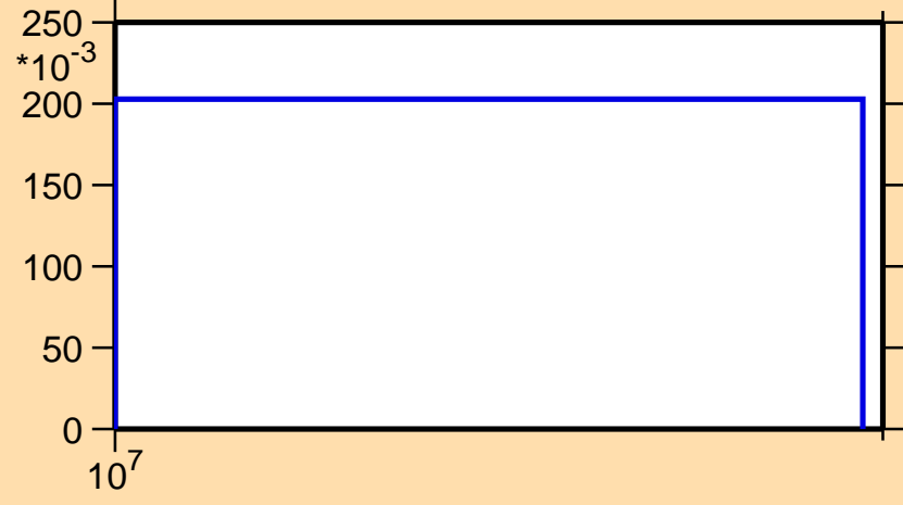
\sigma vs. E for ^{193}\text{Os}(n,3n)
