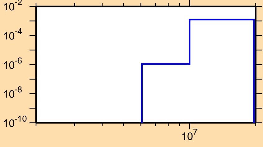
\sigma vs. E for ^{193}\text{Os}(n,p)
