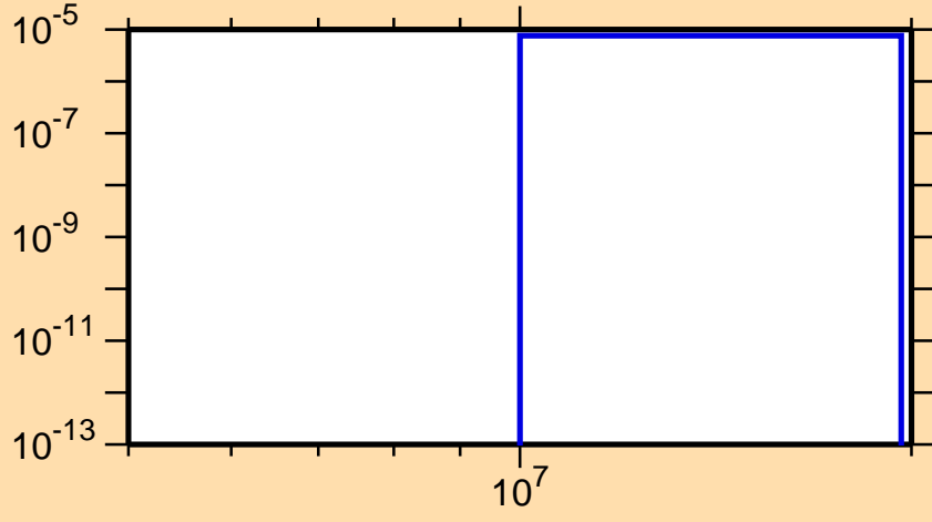
\sigma vs. E for ^{193}\text{Os}(n,np)
