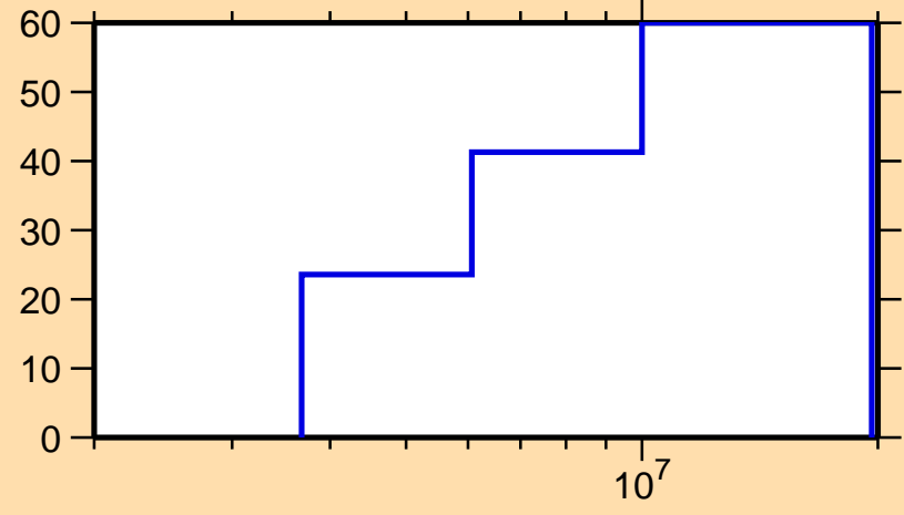
\Delta\sigma/\sigma vs. E for ^{193}\text{Os}(n,ncont.)
