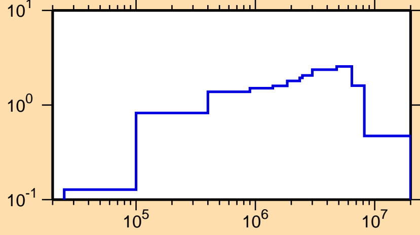
\sigma vs. E for ^{193}\text{Os}(n,\text{inel.})
