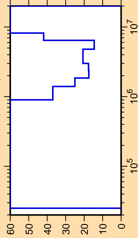
\Delta\sigma/\sigma vs. E for ^{193}\text{Os}(n,\text{inel.})
