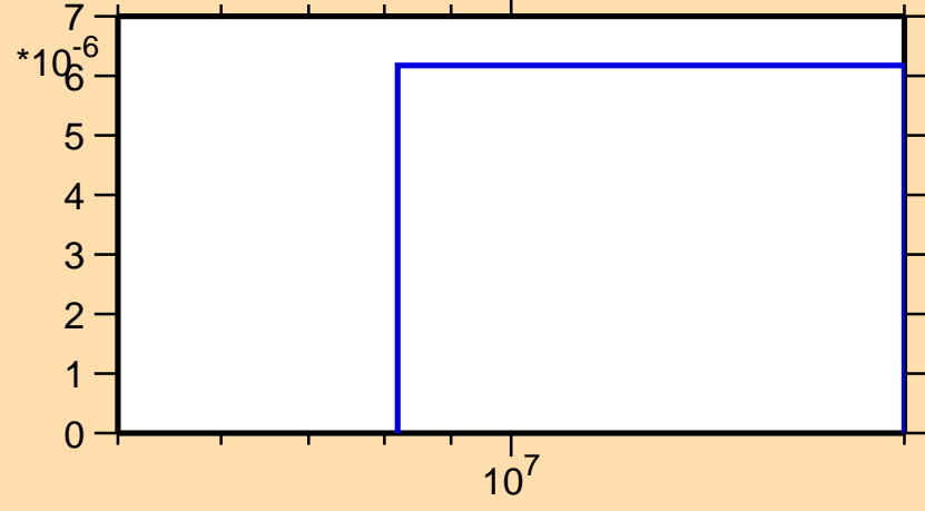
\sigma vs. E for ^{193}\text{Os}(n,np)
