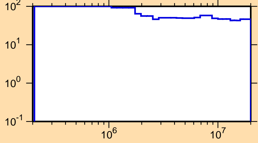
\Delta\sigma/\sigma vs. E for ^{194}\text{Os}(n,n_1)
