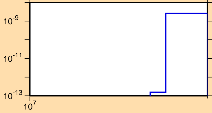
\sigma vs. E for ^{194}\text{Os}(n,nt)
