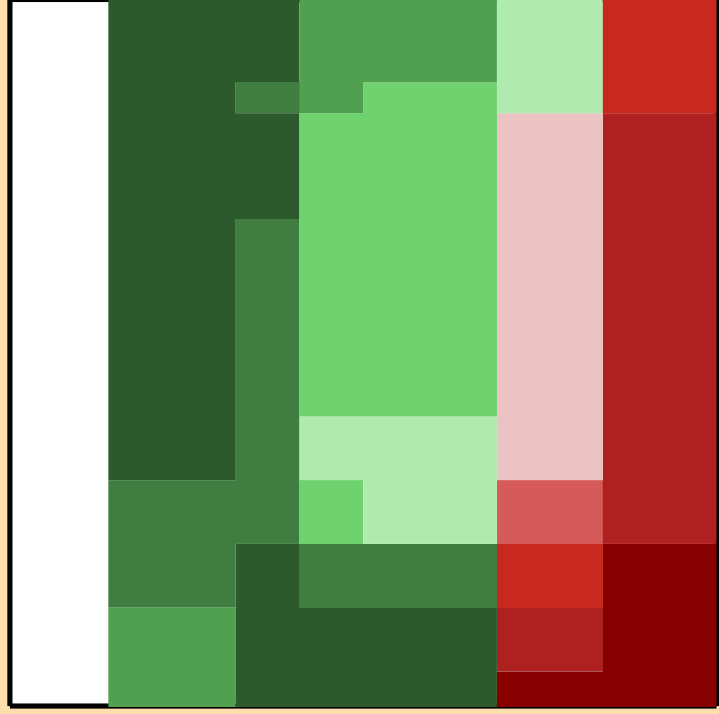
\Delta\sigma/\sigma vs. E for ^{194}\text{Os}(n,p)
