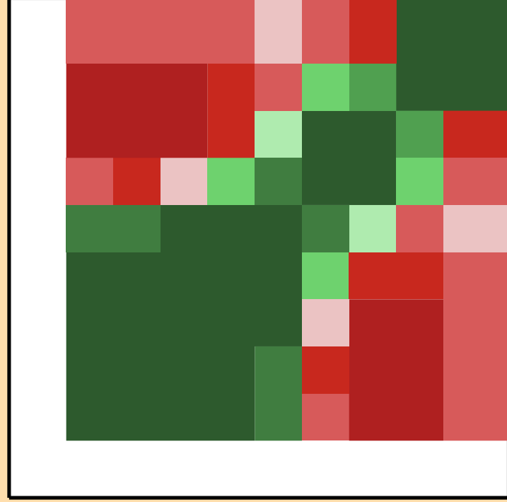
\sigma vs. E for ^{194}\text{Os}(n,\text{inel.})
