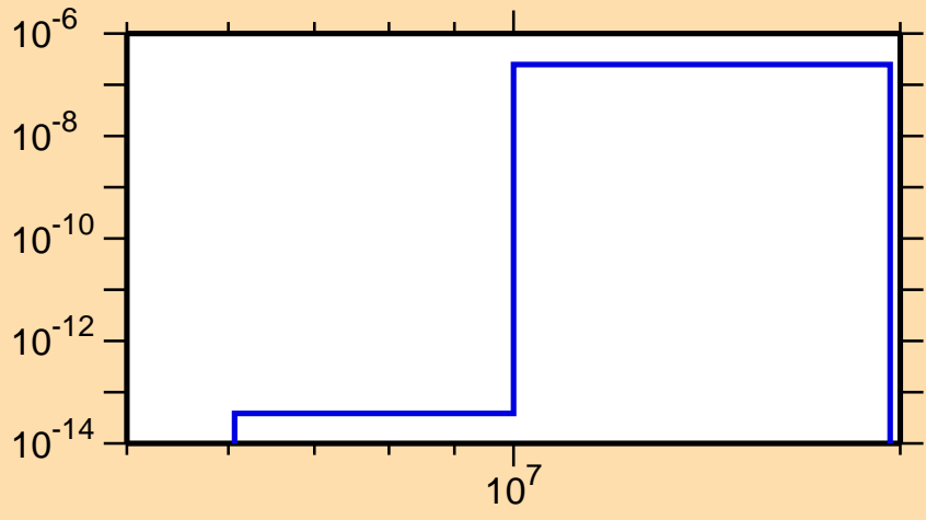
\sigma vs. E for ^{194}\text{Os}(n,n\alpha)
