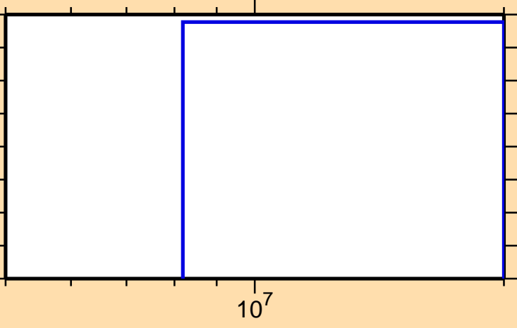
\sigma vs. E for ^{194}\text{Os}(n,3n)
