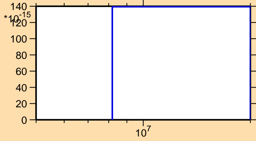
\sigma vs. E for ^{194}\text{Os}(n,2np)
