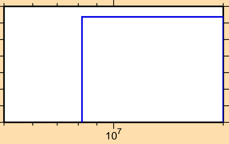
\sigma vs. E for ^{194}\text{Os}(n,np)
