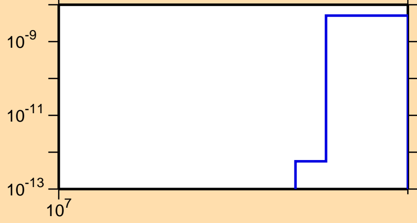
\sigma vs. E for ^{195}\text{Os}(n,nt)
