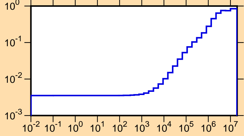
\mu vs. E for ^{195}\text{Os}(\text{mt251})
