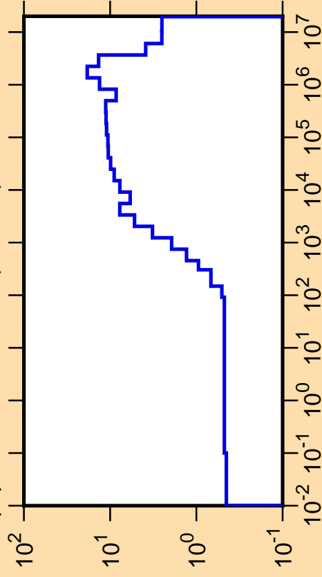
\Delta\mu/\mu vs. E for ^{195}\text{Os}(\text{mt251})
