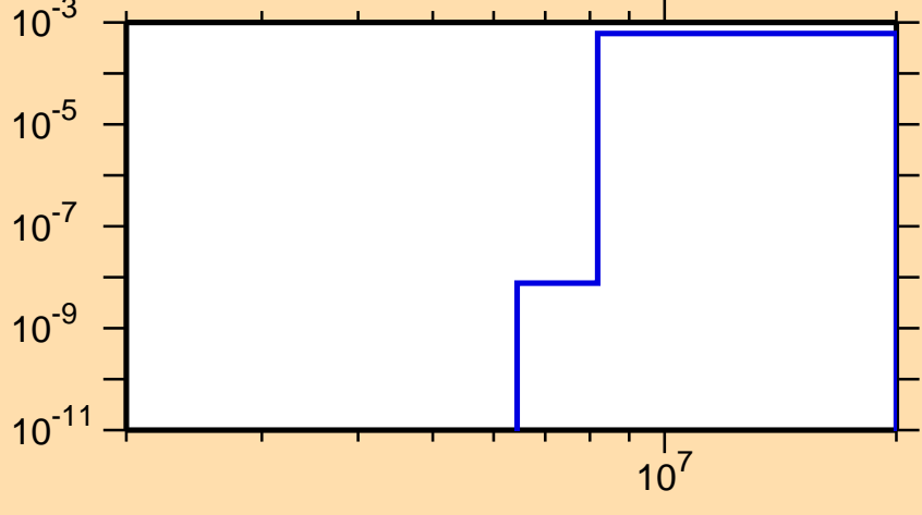
\sigma vs. E for ^{195}\text{Os}(n,p)
