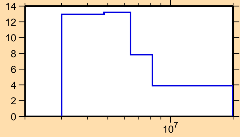
\Delta\sigma/\sigma vs. E for ^{195}\text{Os}(n,el.)
