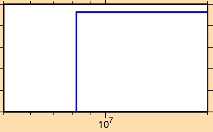
\sigma vs. E for ^{195}\text{Os}(n,\text{nd})
