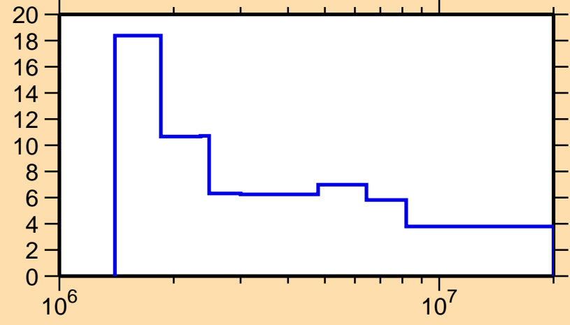
\Delta\sigma/\sigma vs. E for ^{195}\text{Os}(n,n\text{onel.})
