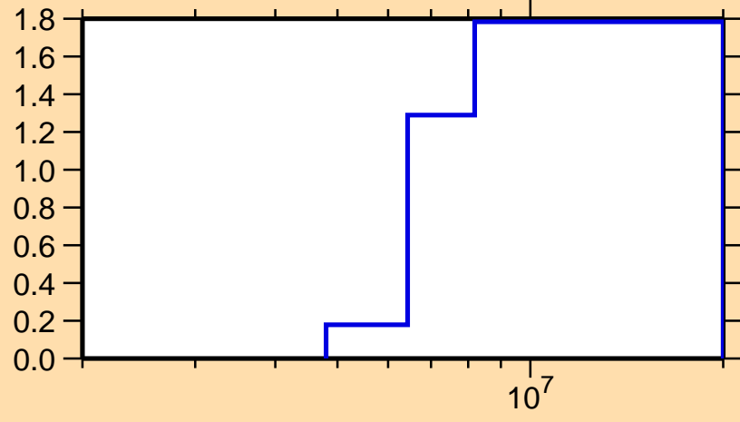
\sigma vs. E for ^{195}\text{Os}(n,2n)
