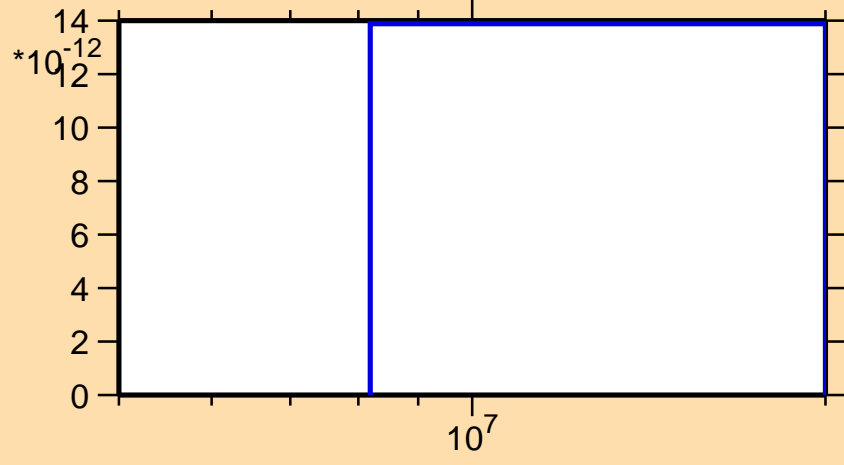
\sigma vs. E for ^{195}\text{Os}(n,2n\alpha)
