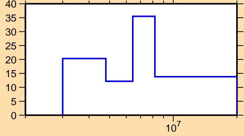
\Delta\sigma/\sigma vs. E for ^{195}\text{Os}(n,ncont.)
