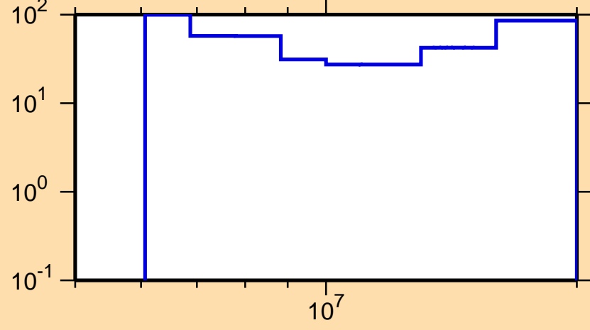
\Delta\sigma/\sigma vs. E for ^{196}\text{Os}(n,2n)
