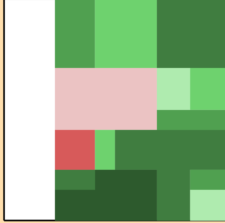
\Delta\sigma/\sigma vs. E for ^{196}\text{Os}(n,2n)
