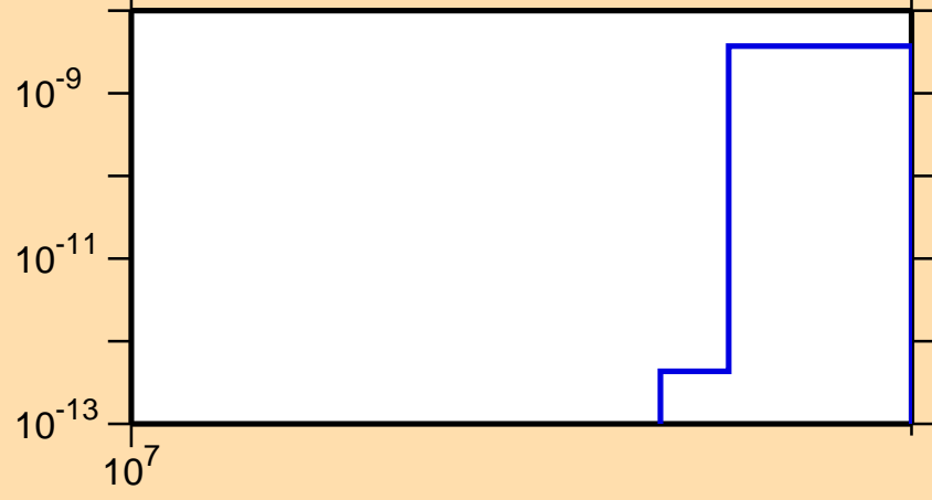
\sigma vs. E for ^{196}\text{Os}(n,nt)
