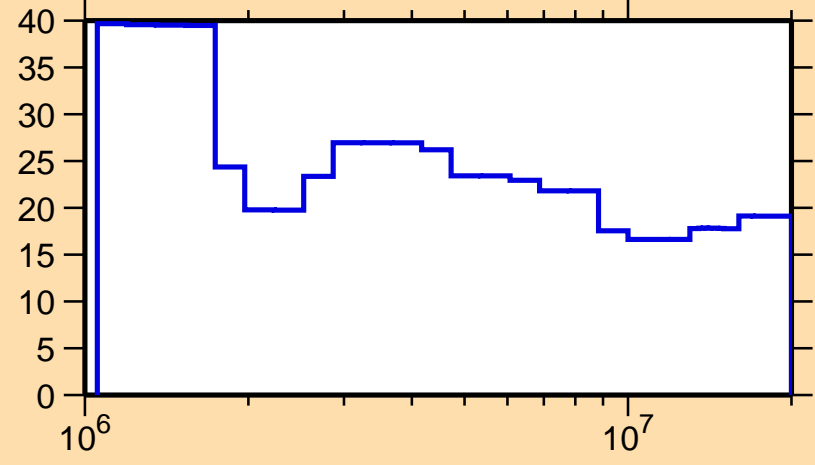
\Delta\sigma/\sigma vs. E for ^{196}\text{Os}(n,n\text{onel.})
