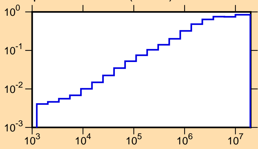
\mu vs. E for ^{196}\text{Os}(\text{mt251})
