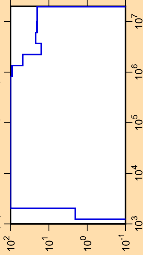
\Delta\mu/\mu vs. E for ^{196}\text{Os}(\text{mt251})
