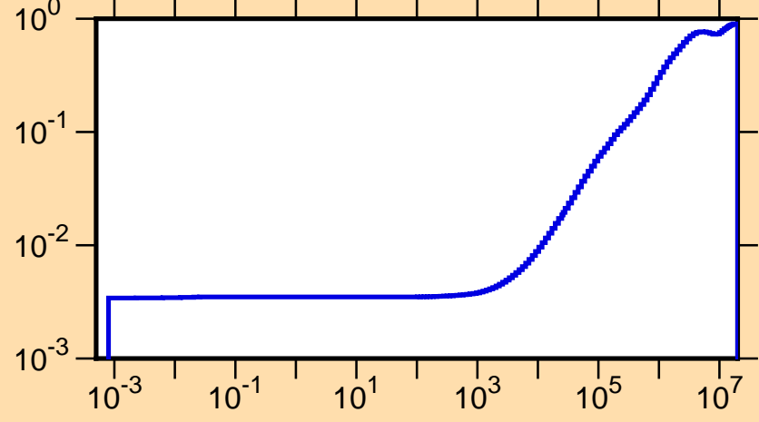
\mu vs. E for ^{197}\text{Os}(\text{mt251})
