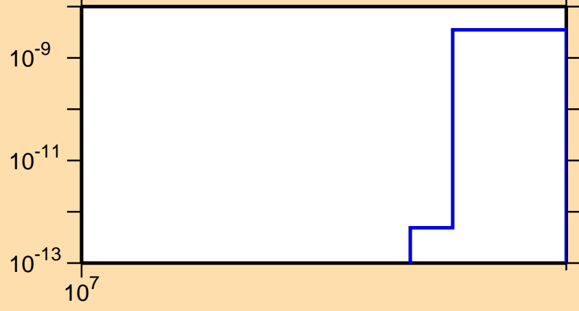
\sigma vs. E for ^{197}\text{Os}(n,nt)
