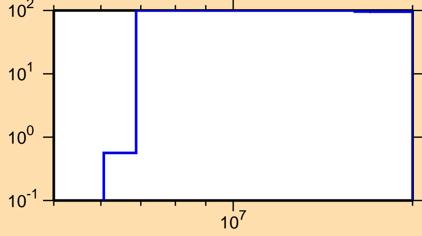
\Delta\sigma/\sigma vs. E for ^{197}\text{Os}(n,p)
