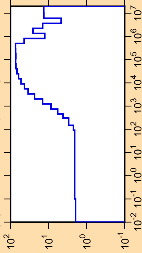
\Delta\mu/\mu vs. E for ^{197}\text{Os}(\text{mt251})
