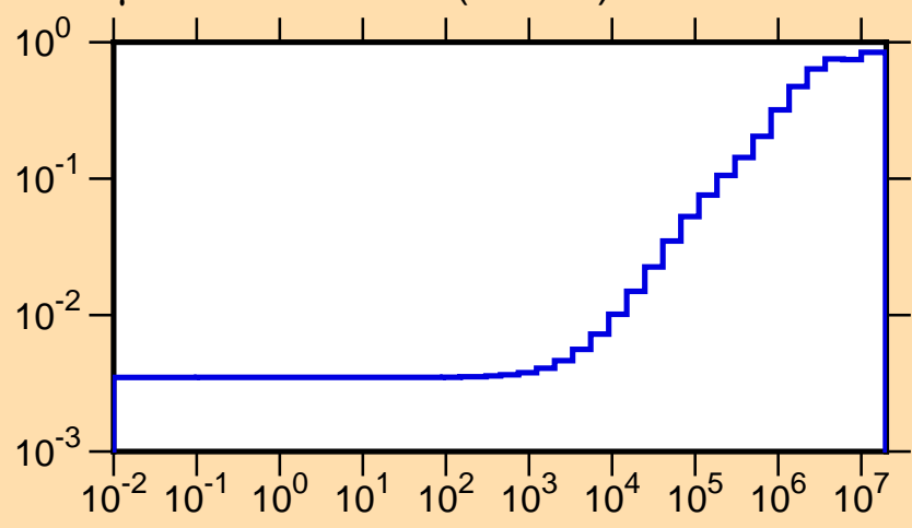
\mu vs. E for ^{197}\text{Os}(\text{mt251})
