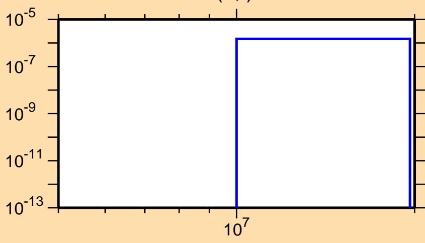
\sigma vs. E for ^{197}\text{Os}(n,t)
