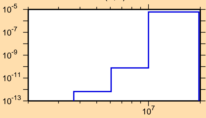
\sigma vs. E for ^{197}\text{Os}(n,\alpha)
