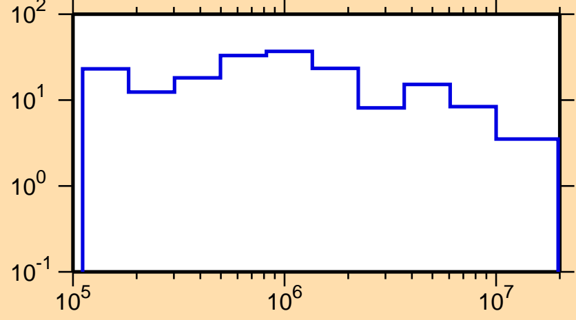
\Delta\sigma/\sigma vs. E for ^{197}\text{Os}(n,\text{tot.})
