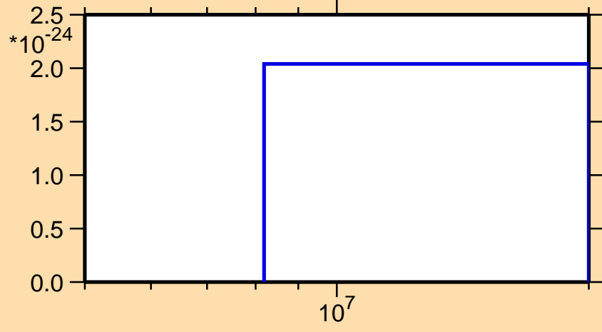
\sigma vs. E for ^{197}\text{Os}(\text{mt } 11)
