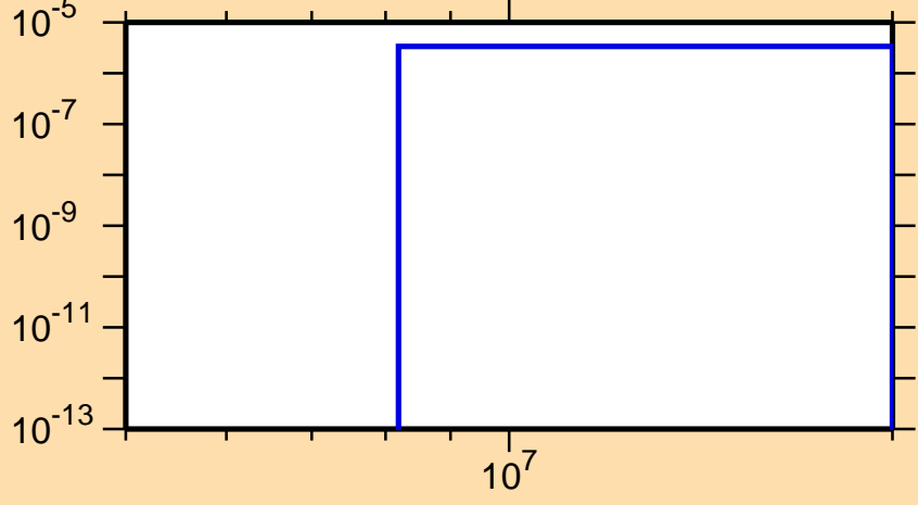
\sigma vs. E for ^{197}\text{Os}(n,d)
