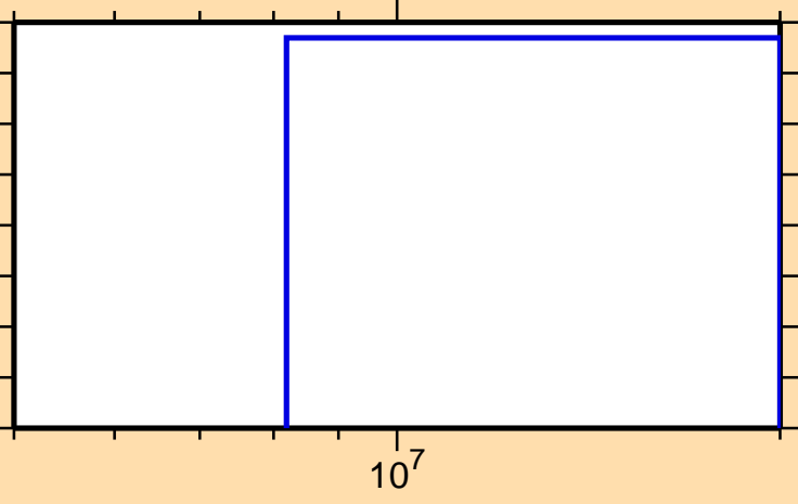
\sigma vs. E for ^{197}\text{Os}(n,\text{nd})
