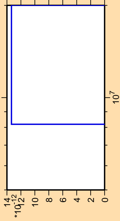
\Delta\sigma/\sigma vs. E for ^{197}\text{Os}(\text{mt } 11)
