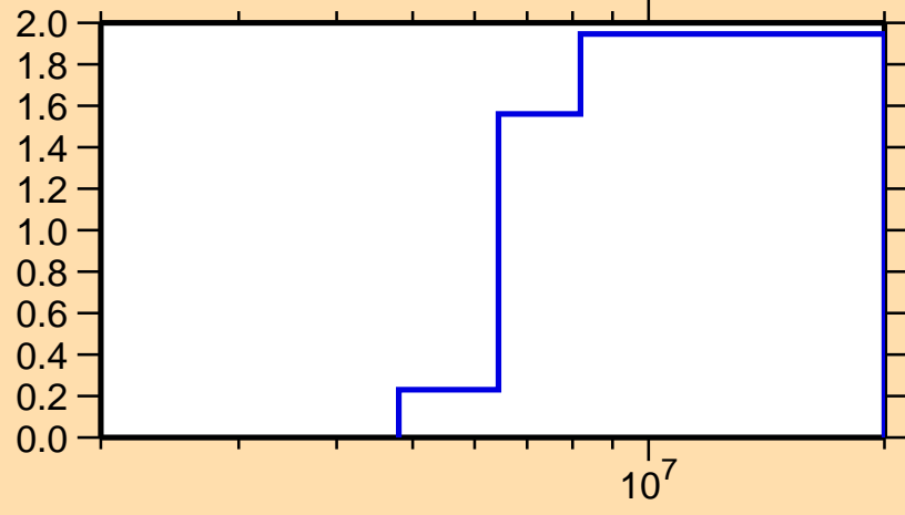
\sigma vs. E for ^{197}\text{Os}(n,2n)
