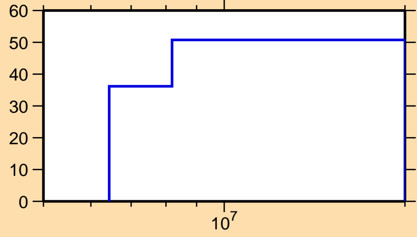
\Delta\sigma/\sigma vs. E for ^{197}\text{Os}(n,ncont.)
