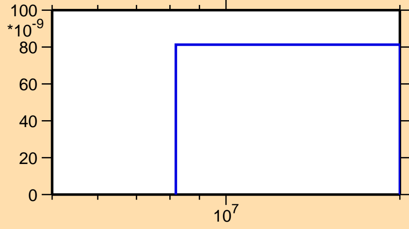
\sigma vs. E for ^{197}\text{Os}(n,n\alpha)
