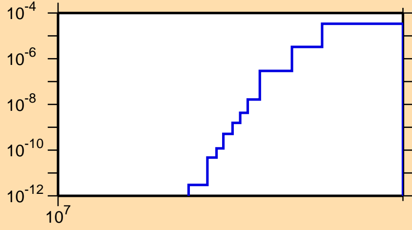
\sigma vs. E for ^{198}\text{Os}(n,np)
