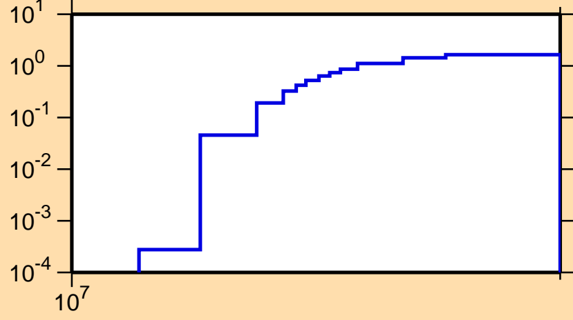
\sigma vs. E for ^{198}\text{Os}(n,3n)
