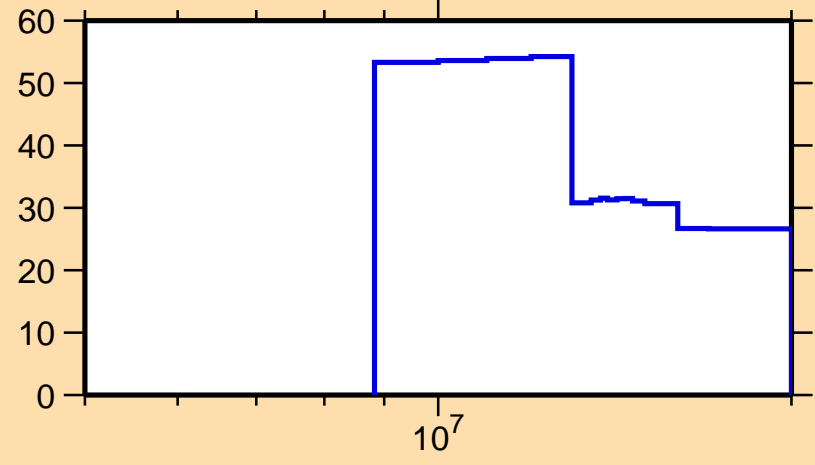
\Delta\sigma/\sigma vs. E for ^{198}\text{Os}(n,ncont.)
