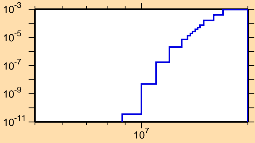
\sigma vs. E for ^{198}\text{Os}(n,p)
