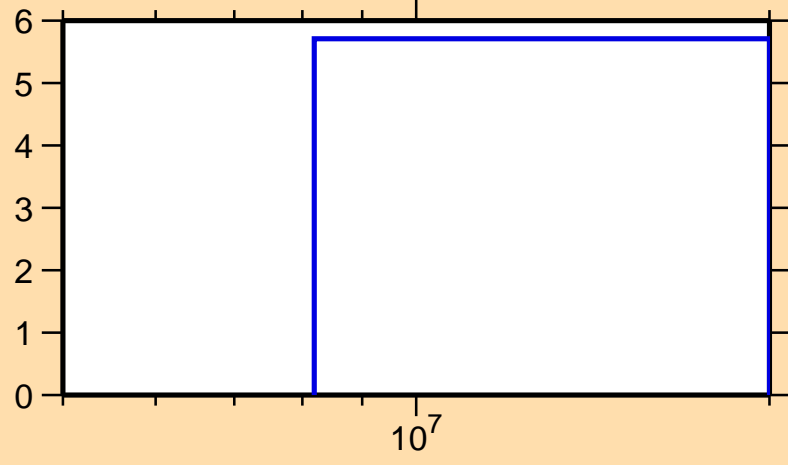
\Delta\sigma/\sigma vs. E for ^{198}\text{Os}(n,el.)
