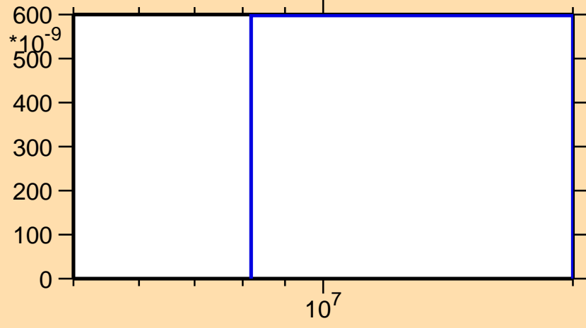
\sigma vs. E for ^{198}\text{Os}(n,d)
