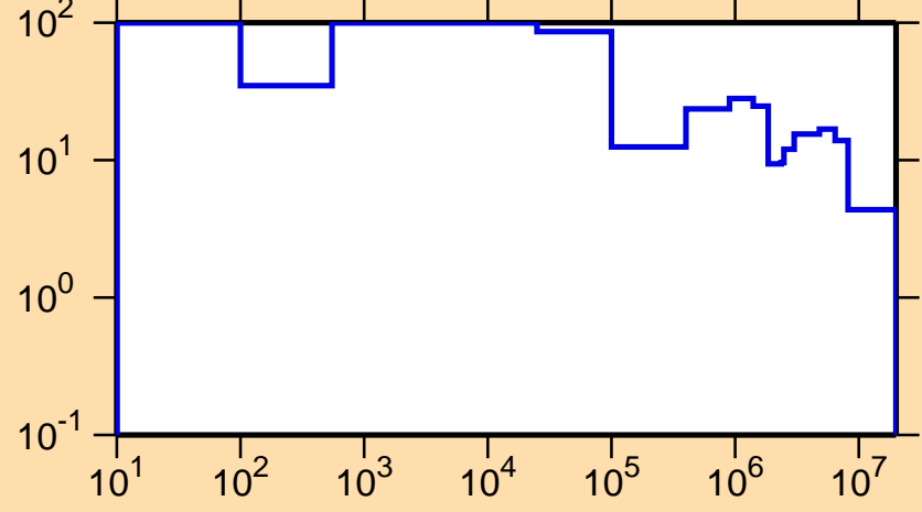
\Delta\sigma/\sigma vs. E for ^{198}\text{Os}(n,\text{tot.})
