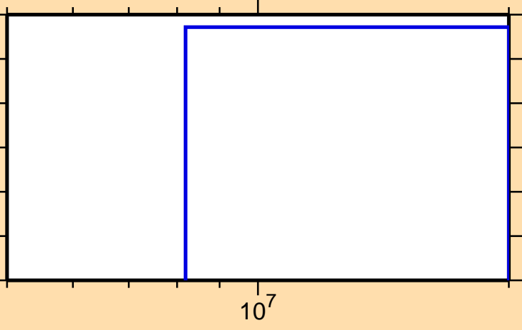
\sigma vs. E for ^{198}\text{Os}(n,p)
