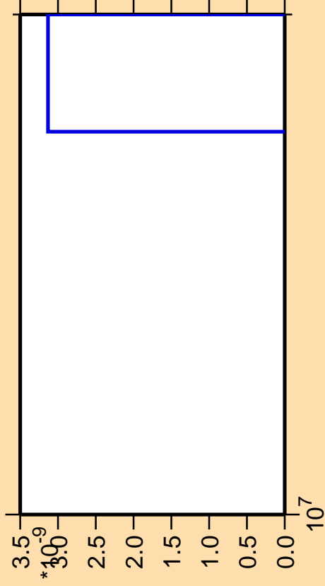
\Delta\sigma/\sigma vs. E for ^{199}\text{Os}(\text{mt } 11)
