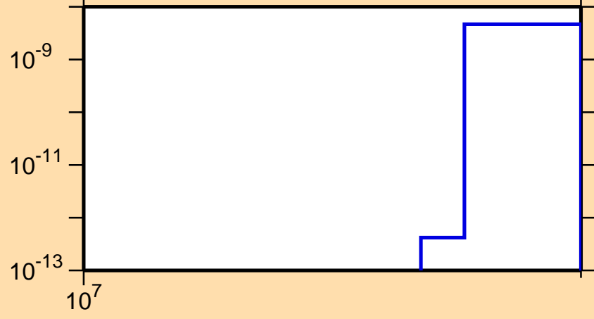
\sigma vs. E for ^{199}\text{Os}(n,nt)
