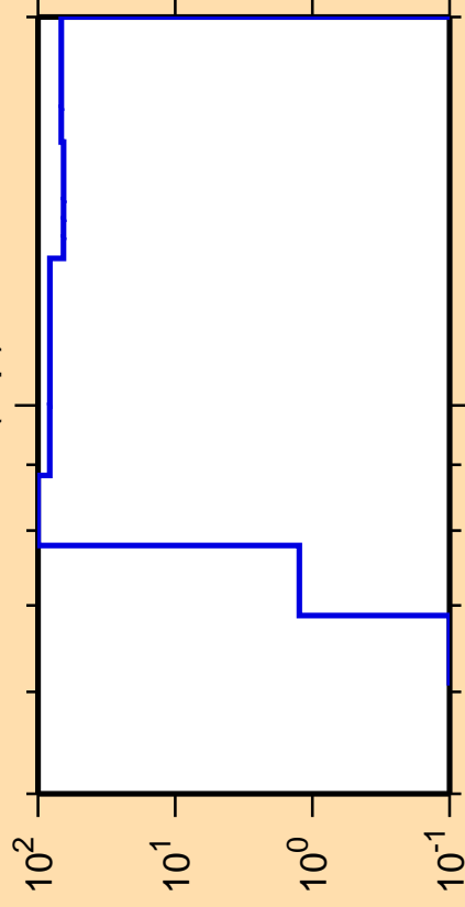
\Delta\sigma/\sigma vs. E for ^{199}\text{Os}(n,p)
