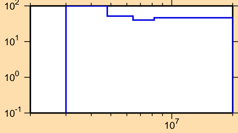
\Delta\sigma/\sigma vs. E for ^{199}\text{Os}(n,2n)
