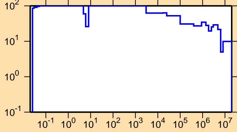
\Delta\sigma/\sigma vs. E for ^{199}\text{Os}(n,\text{tot.})
