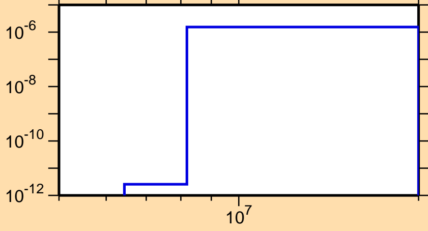
\sigma vs. E for ^{199}\text{Os}(n,\alpha)
