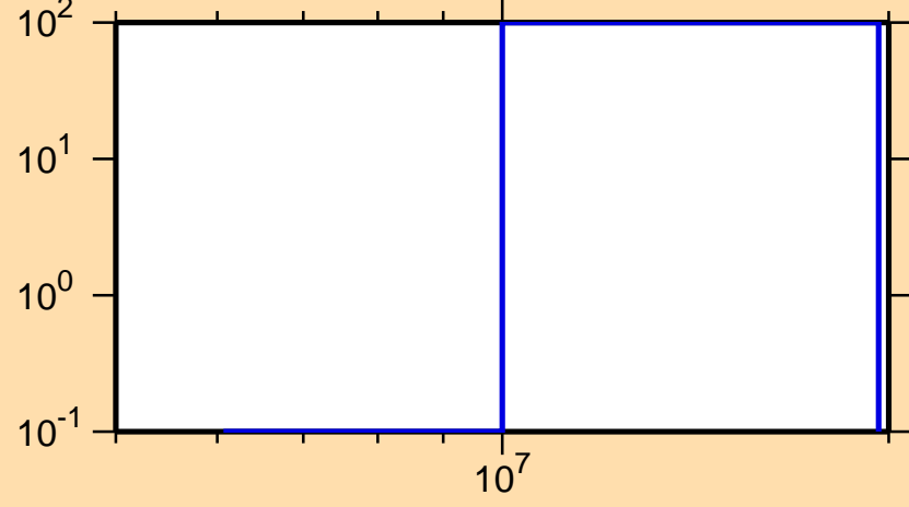
\Delta\sigma/\sigma vs. E for ^{200}\text{Os}(n,p)
