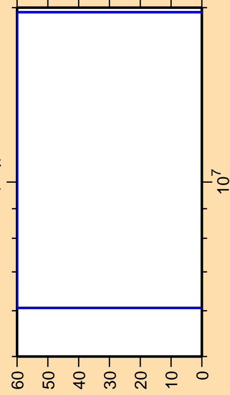
\Delta\sigma/\sigma vs. E for ^{200}\text{Os}(n,\gamma)
