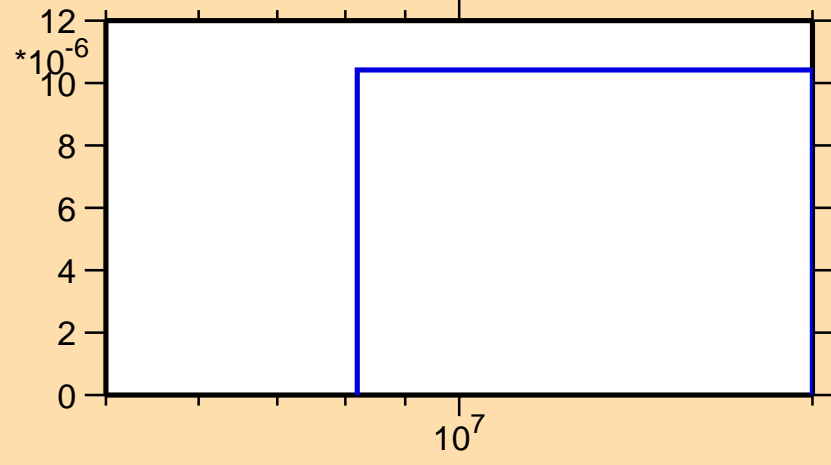
\sigma vs. E for ^{200}\text{Os}(n,p)
