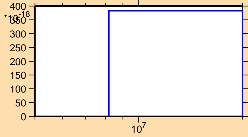
\sigma vs. E for ^{200}\text{Os}(n,2np)
