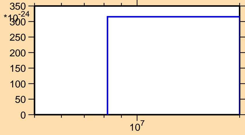
\sigma vs. E for ^{200}\text{Os} (mt 11)
