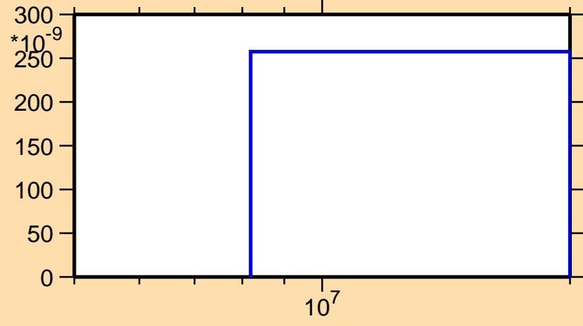
\sigma vs. E for ^{200}\text{Os}(n,\alpha)
