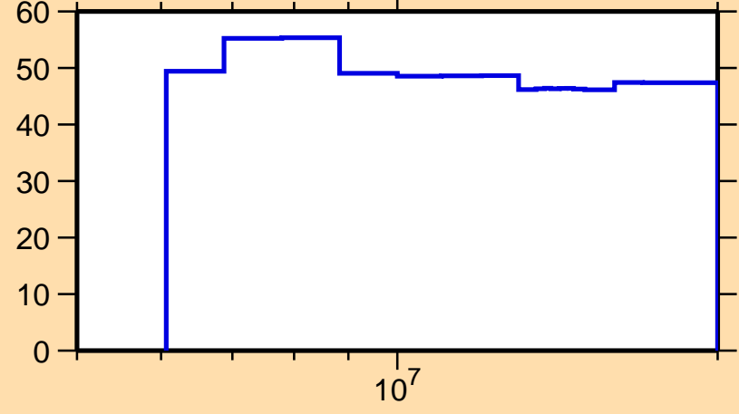
\Delta\sigma/\sigma vs. E for ^{201}\text{Os}(n,ncont.)
