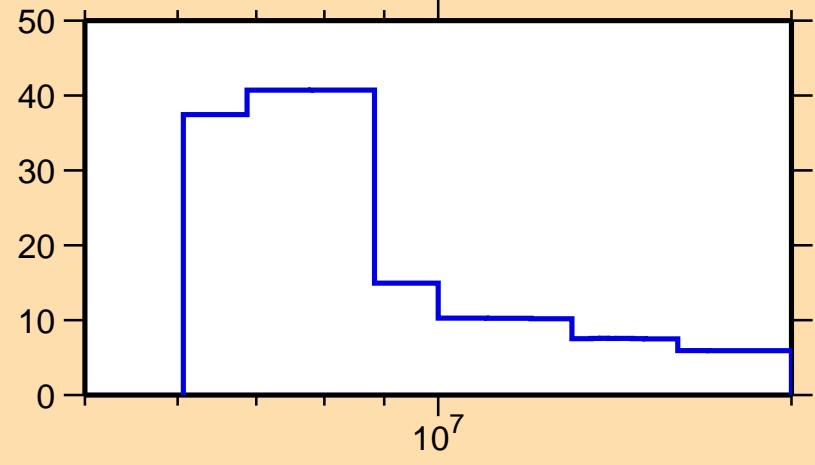
\Delta\sigma/\sigma vs. E for ^{201}\text{Os}(n,el.)
