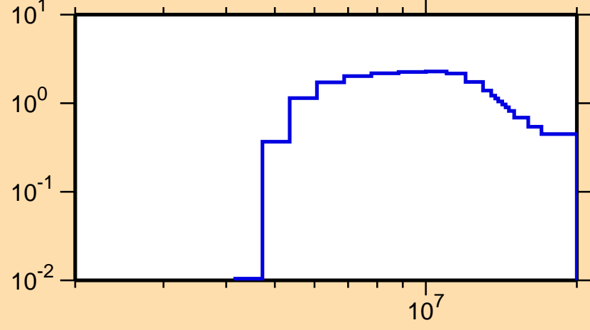
\sigma vs. E for ^{201}\text{Os}(n,2n)
