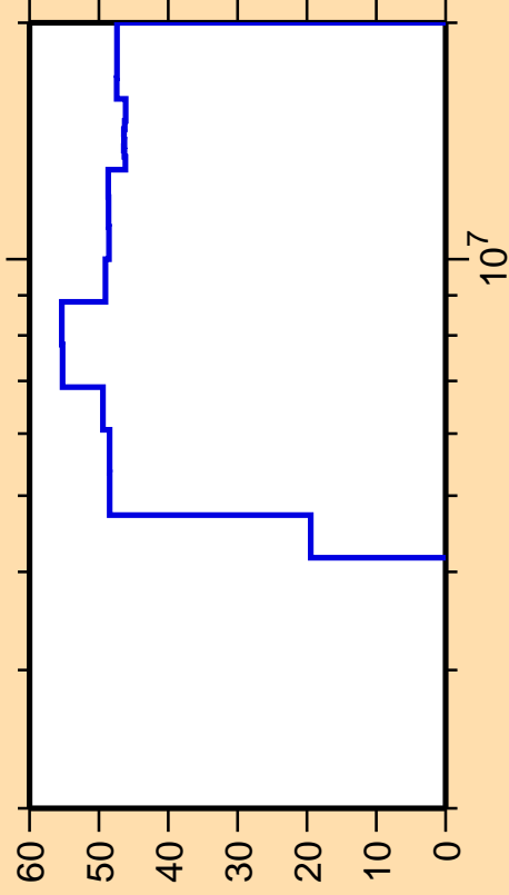
\Delta\sigma/\sigma vs. E for ^{201}\text{Os}(n,n\text{cont.})
