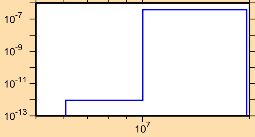
\sigma vs. E for ^{201}\text{Os}(n,\alpha)
