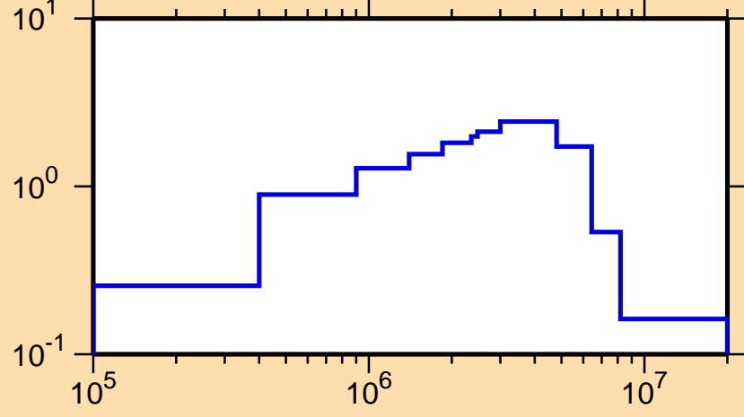
\sigma vs. E for ^{201}\text{Os}(n,\text{inel.})
