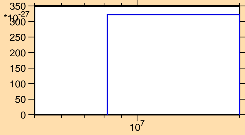
\sigma vs. E for ^{201}\text{Os}(\text{mt } 11)
