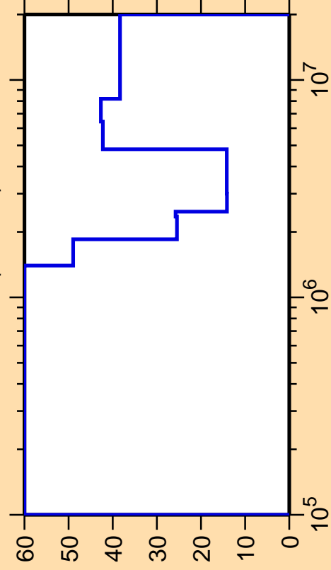
\Delta\sigma/\sigma vs. E for ^{201}\text{Os}(n,\text{inel.})
