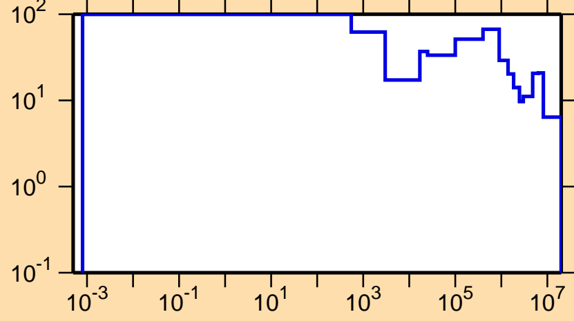
\Delta\sigma/\sigma vs. E for ^{201}\text{Os}(n,tot.)
