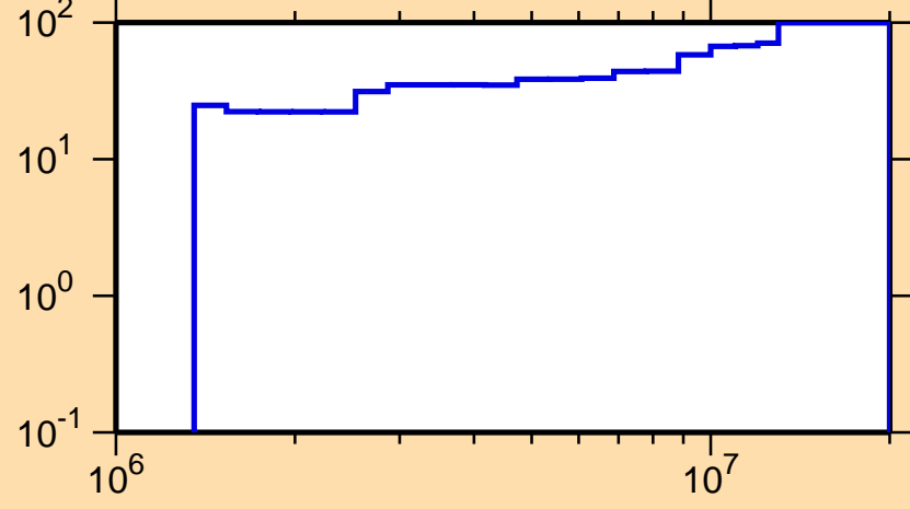
\Delta\sigma/\sigma vs. E for ^{29}\text{P}(n,n_1)
