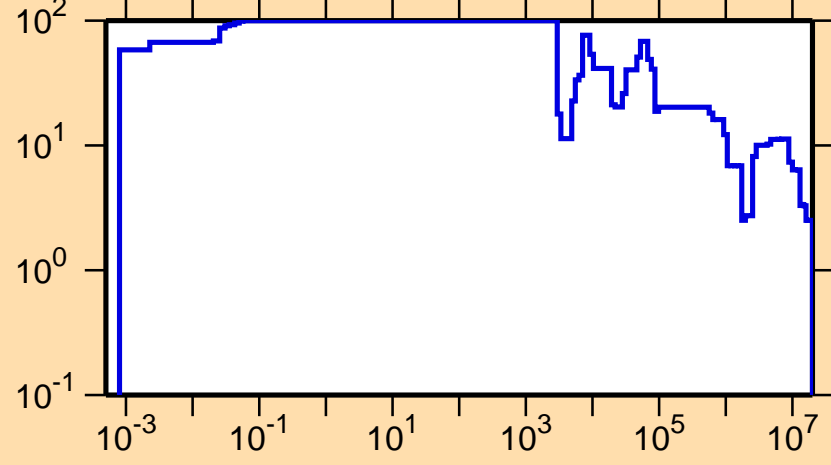
\Delta\sigma/\sigma vs. E for ^{29}\text{P}(n,\text{tot.})
