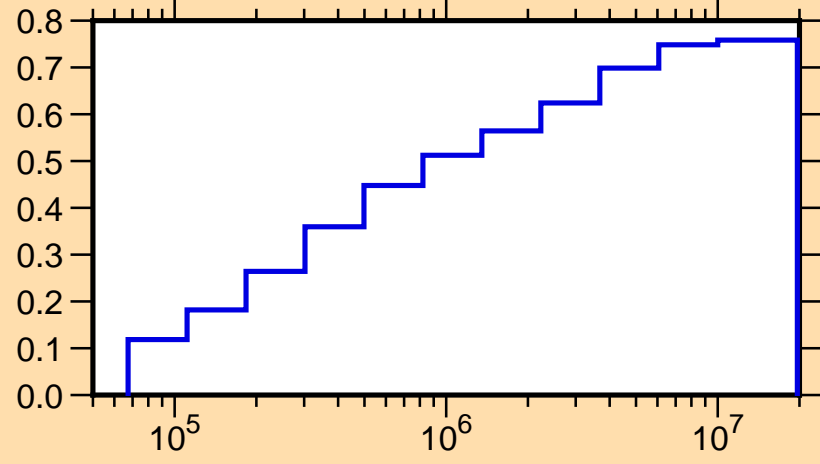
\mu vs. E for ^{29}\text{P}(\text{mt251})
