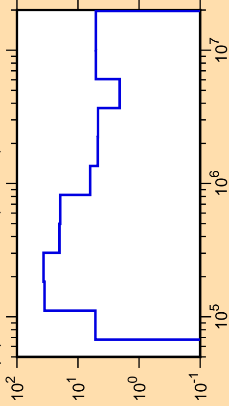
\Delta\mu/\mu vs. E for ^{29}\text{P}(\text{mt251})
