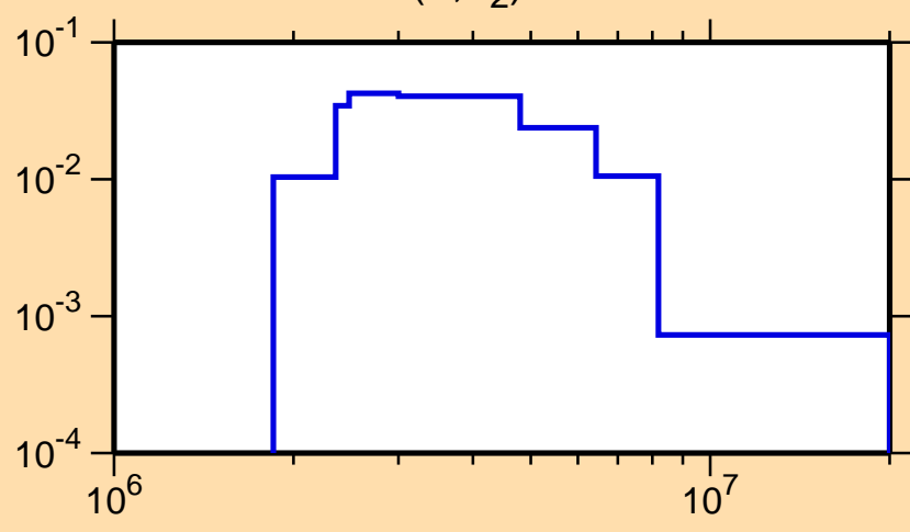
\sigma vs. E for ^{29}\text{P}(n,n_2)
