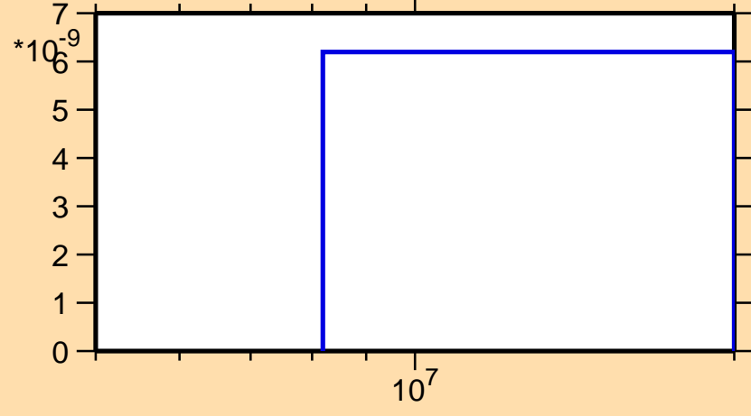
\sigma vs. E for ^{29}\text{P}(n,2n)
