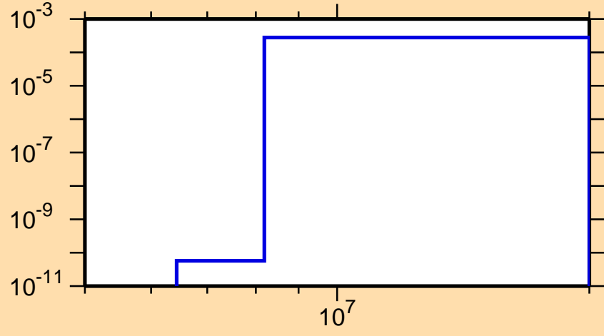
\sigma vs. E for ^{29}\text{P}(n,\text{He}3)
