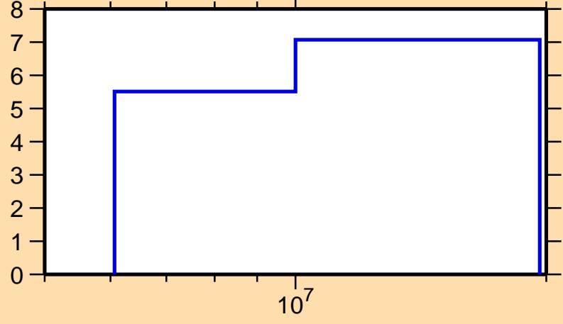
\Delta\sigma/\sigma vs. E for ^{31}\text{P}(n,\text{nonel.})
