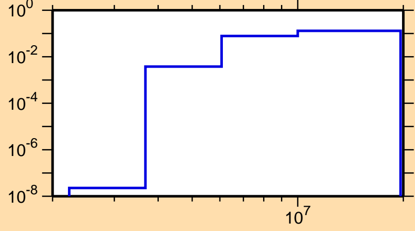
\sigma vs. E for ^{31}\text{P}(n,\alpha)
