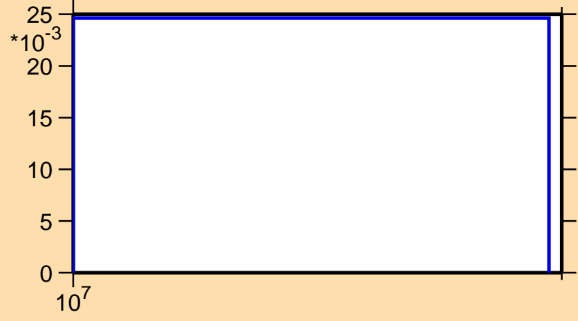
\sigma vs. E for ^{31}\text{P}(n,n\alpha)
