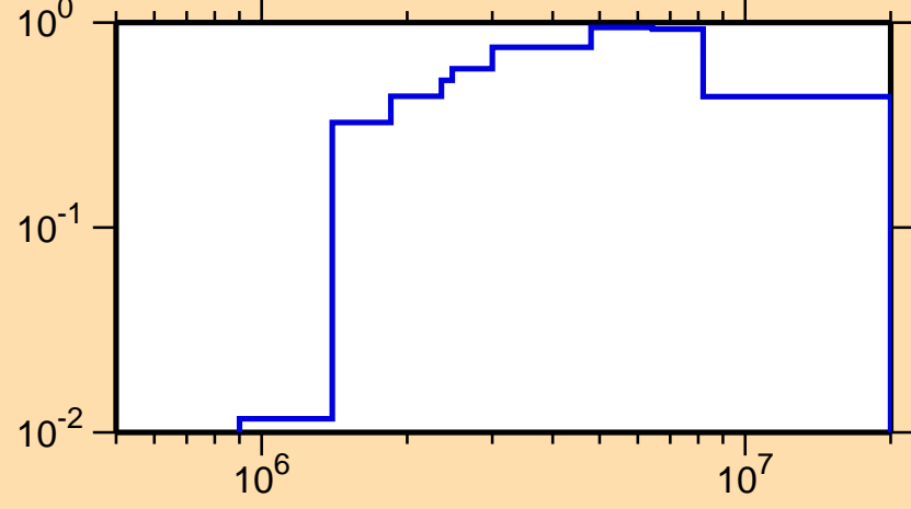
\sigma vs. E for ^{31}\text{P}(n,\text{inel.})
