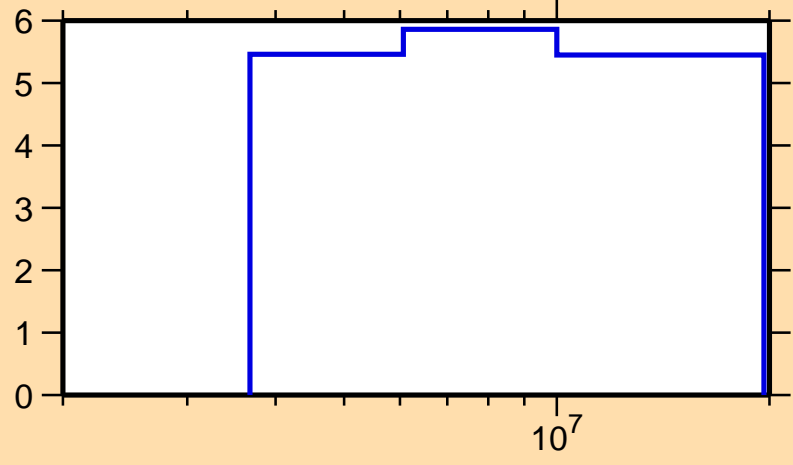
\Delta\sigma/\sigma vs. E for ^{32}\text{P}(n,n\text{onel.})
