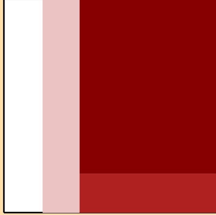
\Delta\sigma/\sigma vs. E for ^{32}\text{P}(n,2n)
