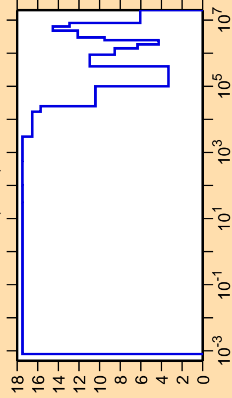
\Delta\sigma/\sigma vs. E for ^{32}\text{P}(n,\text{el.})
