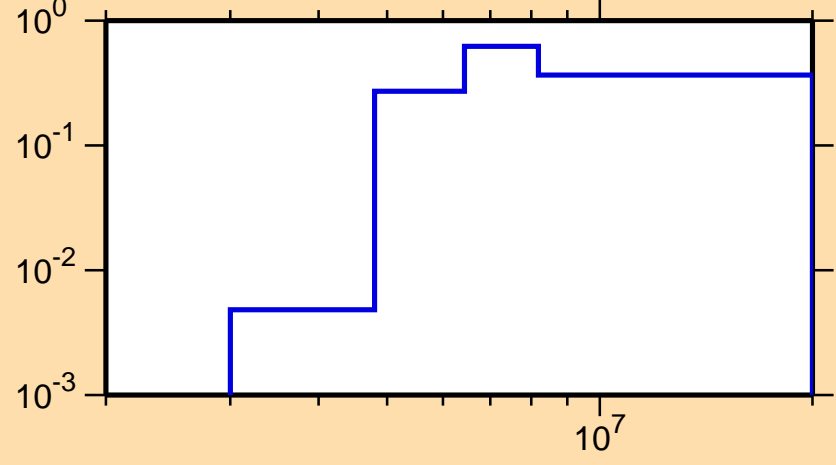
\sigma vs. E for ^{32}\text{P}(n,n\text{cont.})
