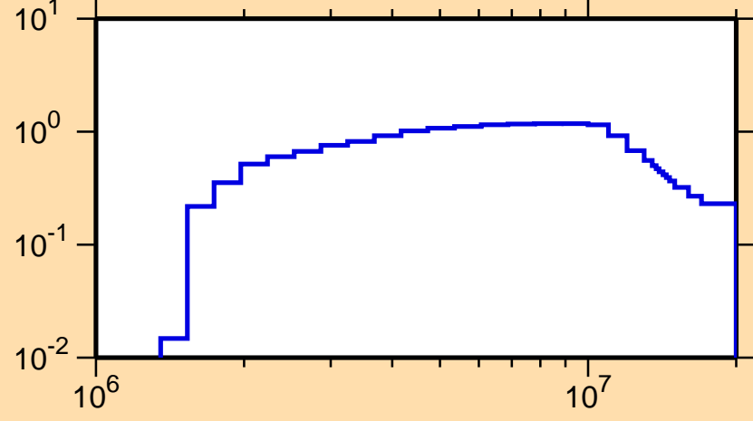
\sigma vs. E for ^{33}\text{P}(n,\text{inel.})
