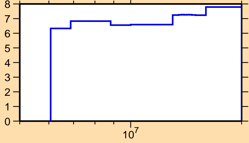
\Delta\sigma/\sigma vs. E for ^{33}\text{P}(n,n\text{onel.})
