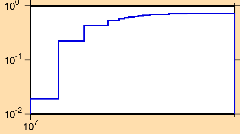
\sigma vs. E for ^{33}\text{P}(n,2n)
