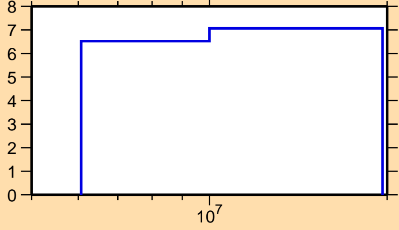
\Delta\sigma/\sigma vs. E for ^{33}\text{P}(n,\text{nonel.})
