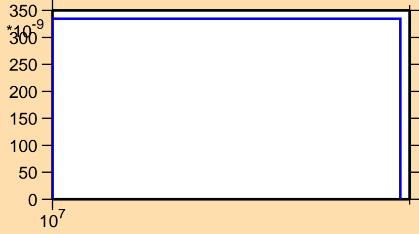
\sigma vs. E for ^{33}\text{P}(n,3n)
