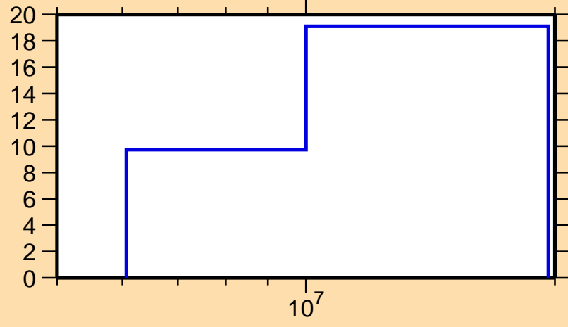
\Delta\sigma/\sigma vs. E for ^{33}\text{P}(n,ncont.)
