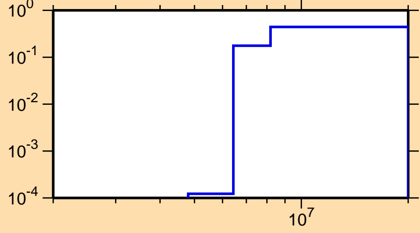
\sigma vs. E for ^{33}\text{P}(n,n\text{cont.})
