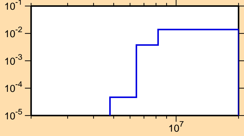
\sigma vs. E for ^{33}\text{P}(n,p)
