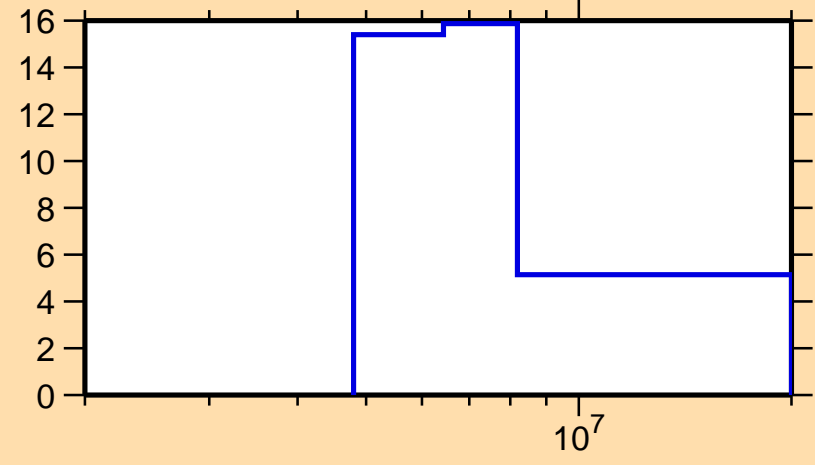
\Delta\sigma/\sigma vs. E for ^{33}\text{P}(n,el.)
