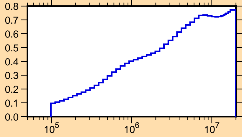
\mu vs. E for ^{34}\text{P}(\text{mt251})
