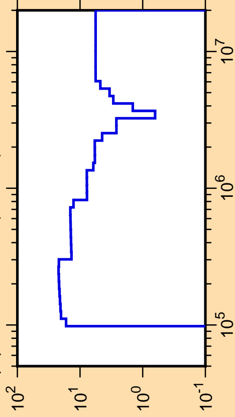
\Delta\mu/\mu vs. E for ^{34}\text{P}(\text{mt251})
