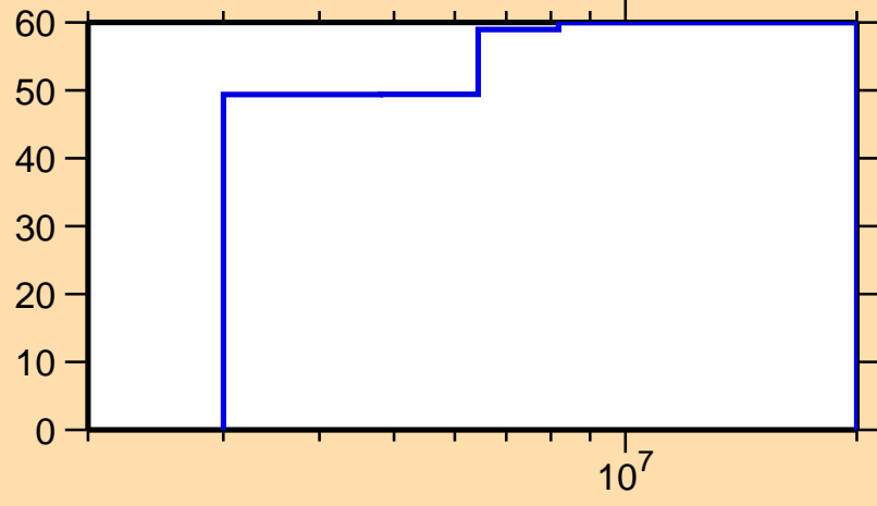
\Delta\sigma/\sigma vs. E for ^{34}\text{P}(n,\gamma)
