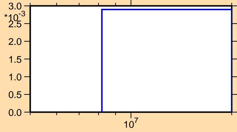
\sigma vs. E for ^{34}\text{P}(n,d)
