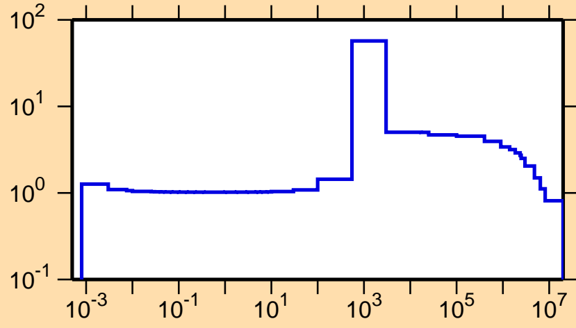
\sigma vs. E for ^{34}\text{P}(n,\text{el.})
