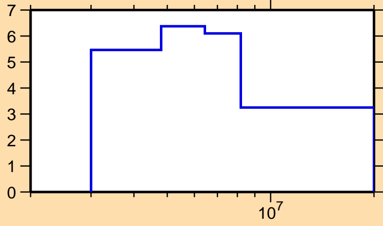
\Delta\sigma/\sigma vs. E for ^{34}\text{P}(n,el.)
