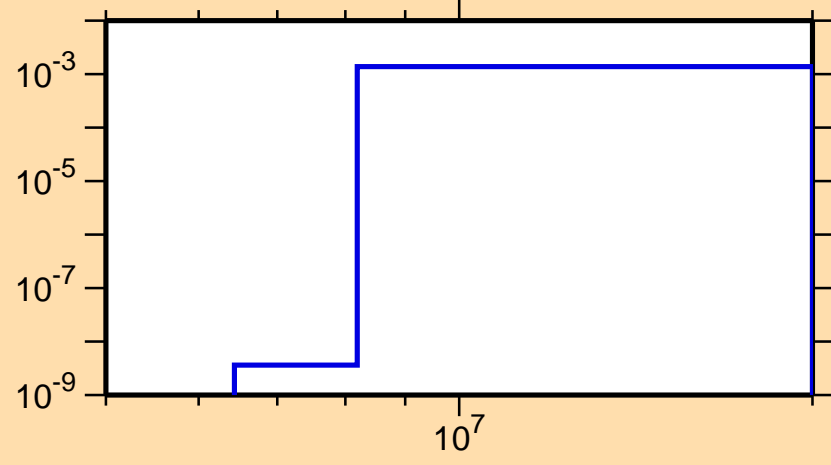
\sigma vs. E for ^{34}\text{P}(n,t)
