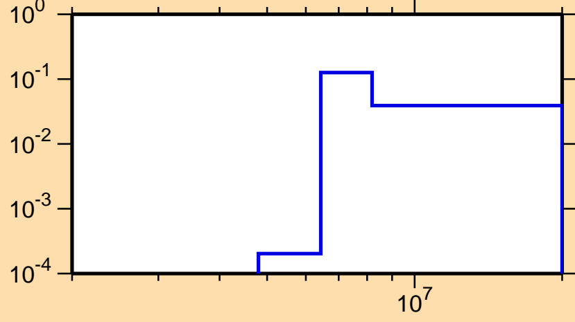
\sigma vs. E for ^{34}\text{P}(n,n\text{cont.})
