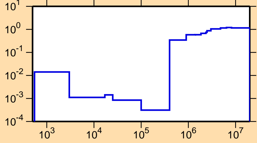
\sigma vs. E for ^{34}\text{P}(n,\text{nonel.})
