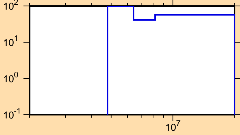
\Delta\sigma/\sigma vs. E for ^{34}\text{P}(n,ncont.)
