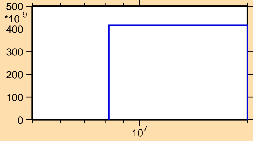
\sigma vs. E for ^{34}\text{P}(n,2np)
