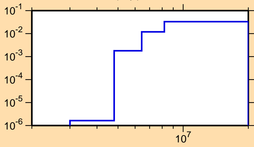
\sigma vs. E for ^{34}\text{P}(n,p)
