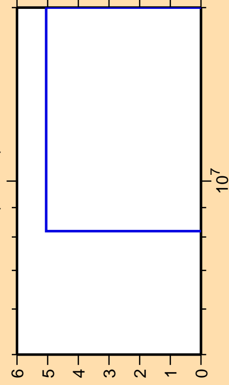
\Delta\sigma/\sigma vs. E for ^{34}\text{P}(n,2n\alpha)
