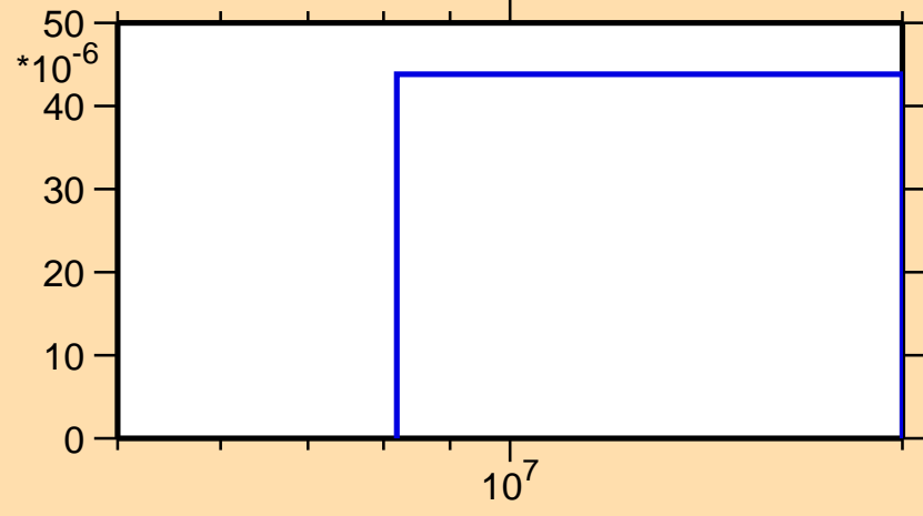
\sigma vs. E for ^{34}\text{P}(n,3n)
