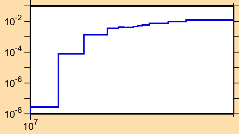
\sigma vs. E for ^{35}\text{P}(n,d)
