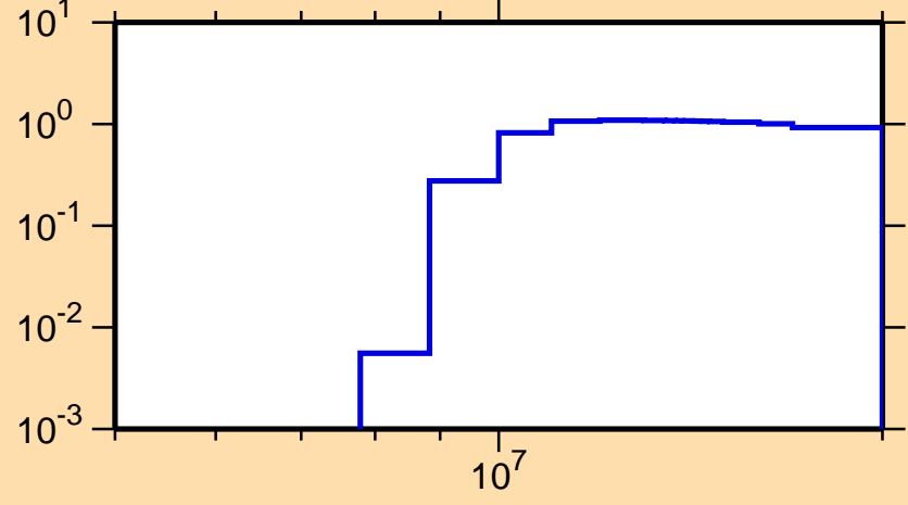
\sigma vs. E for ^{35}\text{P}(n,2n)
