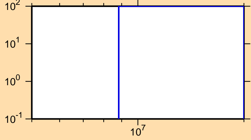
\Delta\sigma/\sigma vs. E for ^{35}\text{P}(n,p)
