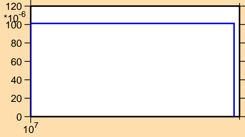
\sigma vs. E for ^{35}\text{P}(n,t)
