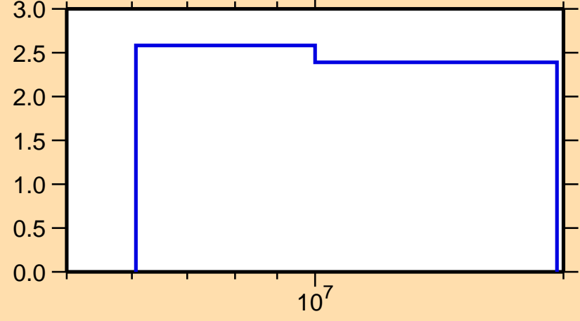
\Delta\sigma/\sigma vs. E for ^{35}\text{P}(n,2n)
