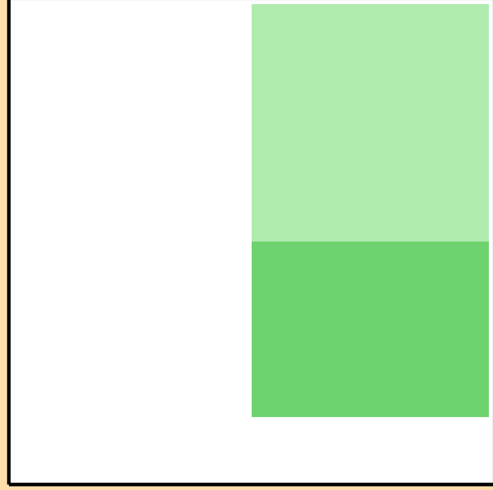
\Delta\sigma/\sigma vs. E for ^{35}\text{P}(n,p)
