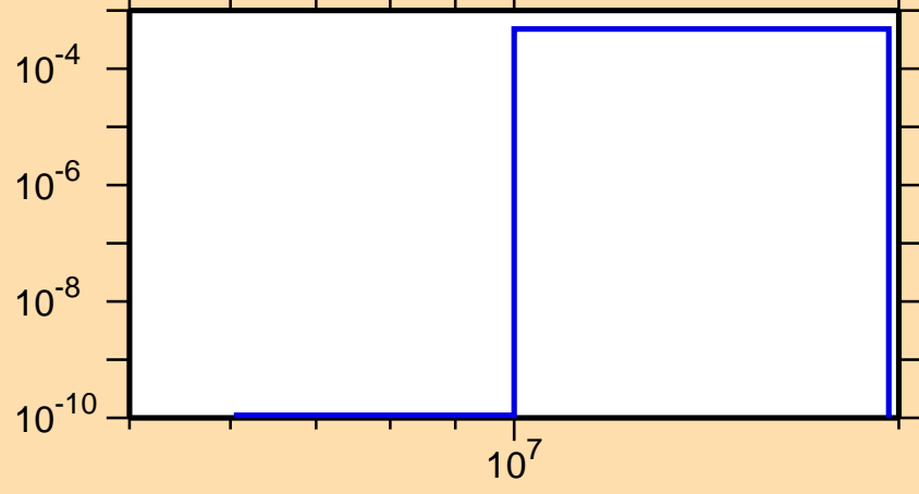
\sigma vs. E for ^{35}\text{P}(n,\alpha)
