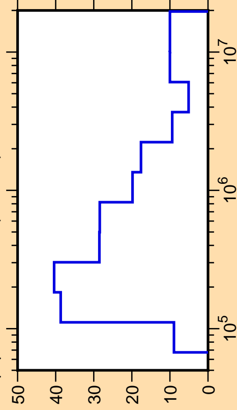
\Delta\mu/\mu vs. E for ^{36}\text{P}(\text{mt251})
