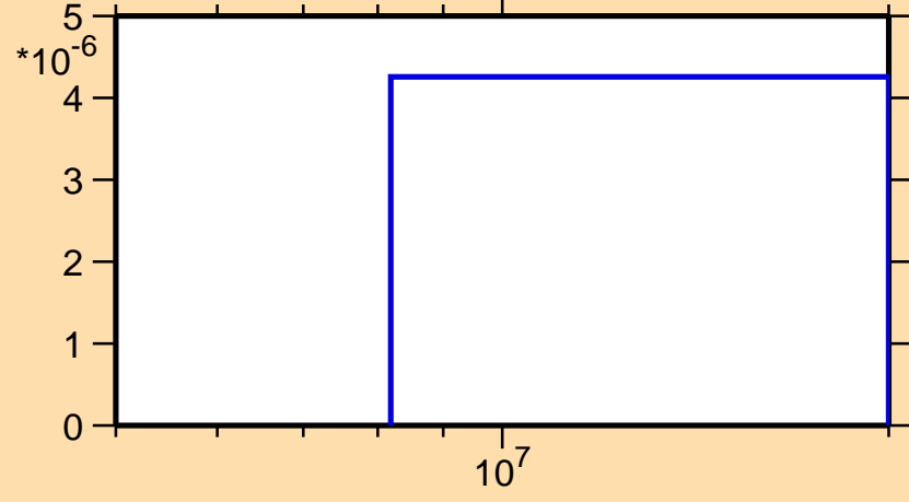
\sigma vs. E for ^{36}\text{P}(n,nd)
