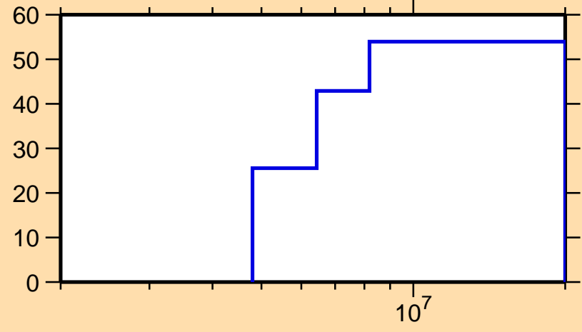
\Delta\sigma/\sigma vs. E for ^{36}\text{P}(n,\text{inel.})
