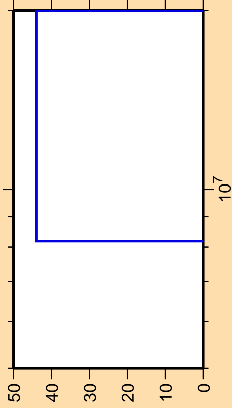
\Delta\sigma/\sigma vs. E for ^{36}\text{P}(n,d)
