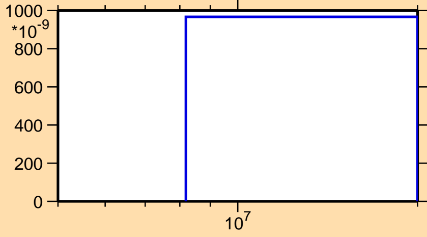
\sigma vs. E for ^{36}\text{P}(n,nt)
