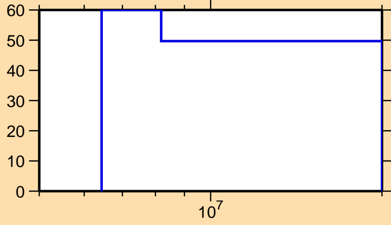
\Delta\sigma/\sigma vs. E for ^{36}\text{P}(n,p)
