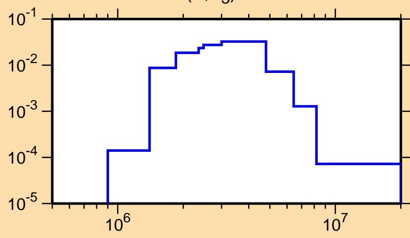
\sigma vs. E for ^{36}\text{P}(n,n_3)
