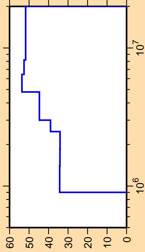
\Delta\sigma/\sigma vs. E for ^{36}\text{P}(n,n_3)
