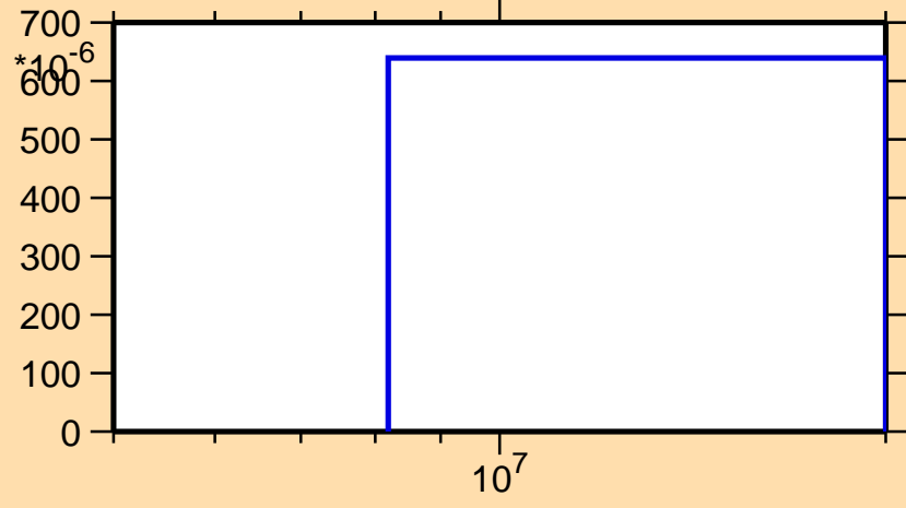
\sigma vs. E for ^{36}\text{P}(n,d)
