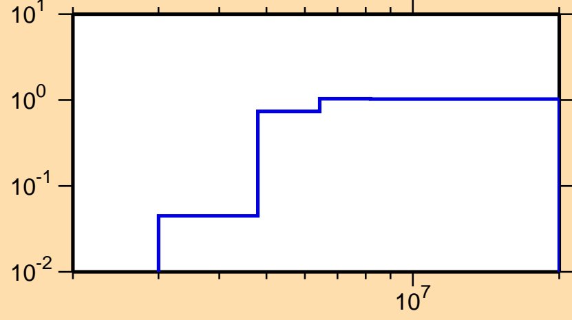
\sigma vs. E for ^{36}\text{P}(n,2n)
