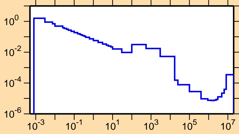
\sigma vs. E for ^{36}\text{P}(n,\gamma)
