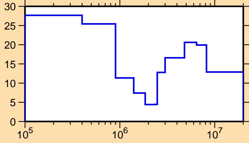
\Delta\sigma/\sigma vs. E for ^{36}\text{P}(n,\text{el.})
