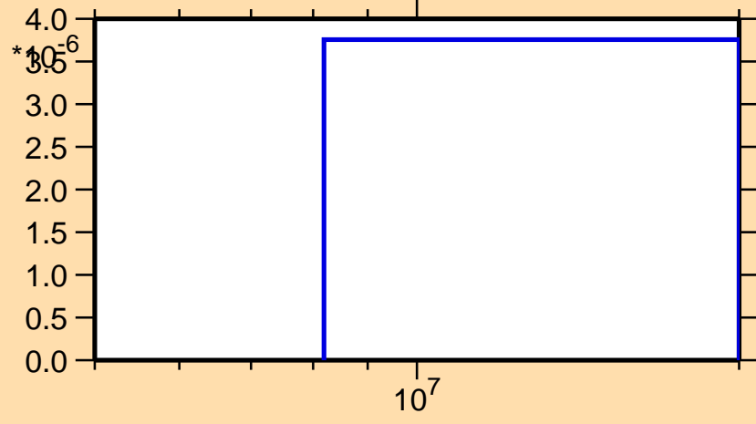
\sigma vs. E for ^{36}\text{P}(n,n\alpha)
