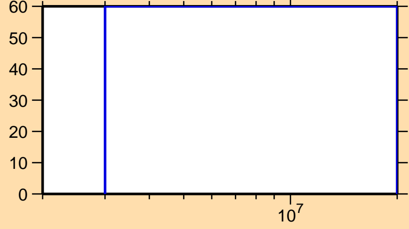
\Delta\sigma/\sigma vs. E for ^{36}\text{P}(n,n\text{cont.})
