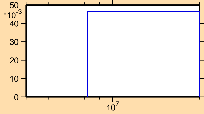
\sigma vs. E for ^{36}\text{P}(n,3n)
