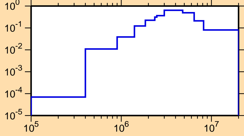
\sigma vs. E for ^{36}\text{P}(n,\text{inel.})
