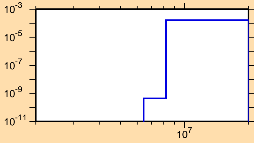
\sigma vs. E for ^{36}\text{P}(n,\alpha)
