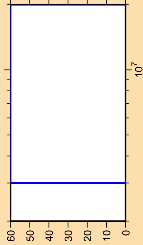
\Delta\sigma/\sigma vs. E for ^{36}\text{P}(n,n\text{cont.})
