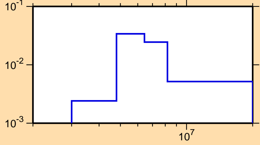
\sigma vs. E for ^{36}\text{P}(n,n\text{cont.})
