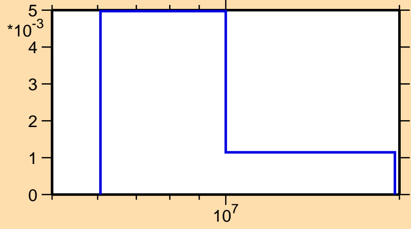
\sigma vs. E for ^{37}\text{P}(n,n\text{cont.})
