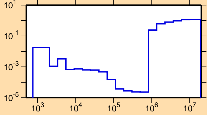
\sigma vs. E for ^{37}\text{P}(n,\text{nonel.})
