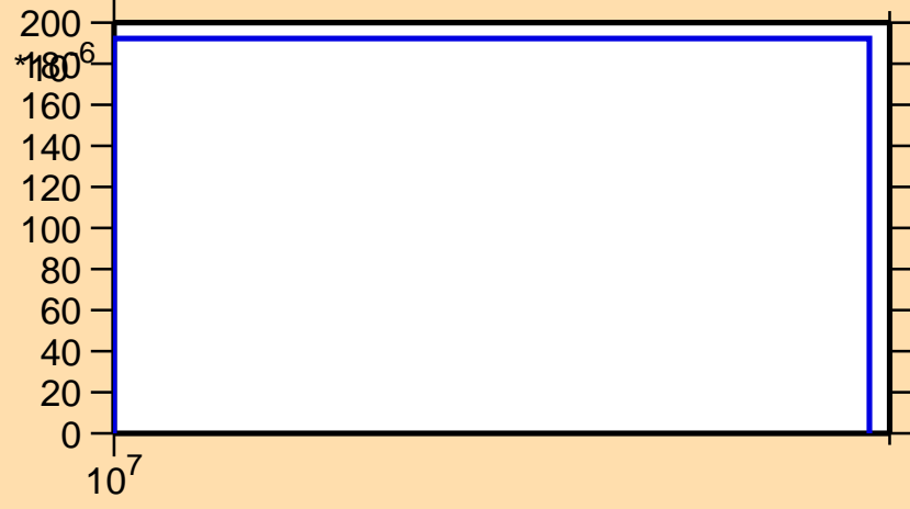
\sigma vs. E for ^{37}\text{P}(n,p)
