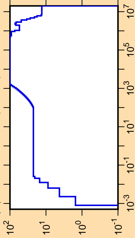
\Delta\mu/\mu vs. E for ^{187}\text{Pb}(\text{mt251})
