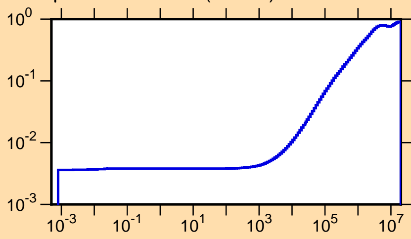
\mu vs. E for ^{187}\text{Pb}(\text{mt251})
