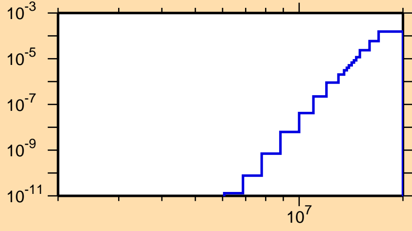
\sigma vs. E for ^{187}\text{Pb}(n,\text{He3})
