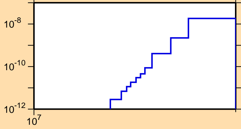
\sigma vs. E for ^{187}\text{Pb}(\text{mt } 34)
