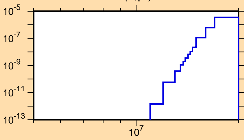
\sigma vs. E for ^{187}\text{Pb}(n,\text{pt})
