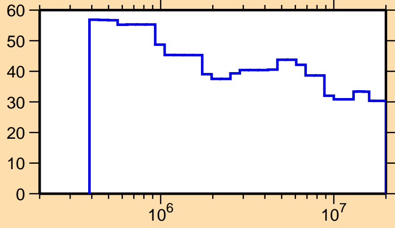
\Delta\sigma/\sigma vs. E for ^{187}\text{Pb}(n,n\text{onel.})
