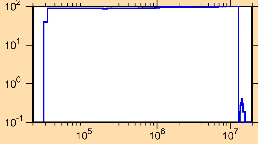
\Delta\sigma/\sigma vs. E for ^{187}\text{Pb}(n,n_1)
