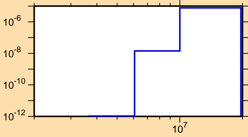
\sigma vs. E for ^{187}\text{Pb}(\text{mt117})
