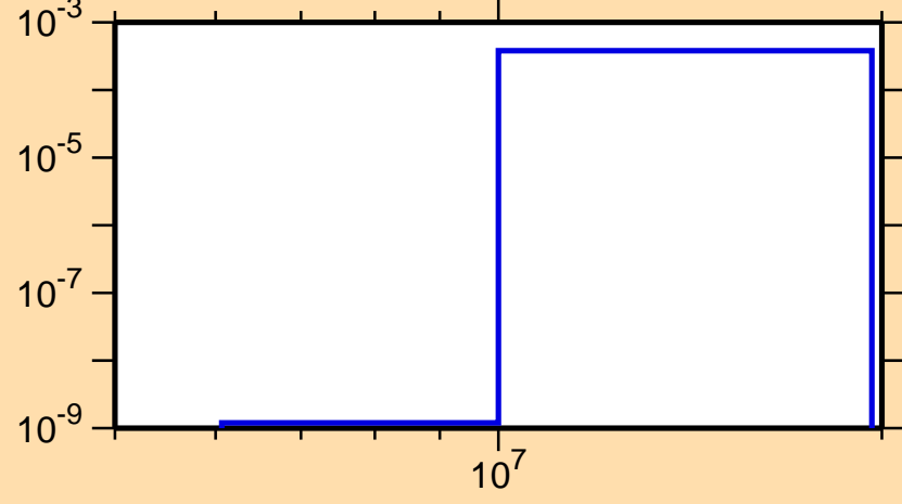
\sigma vs. E for ^{187}\text{Pb}(n,t)
