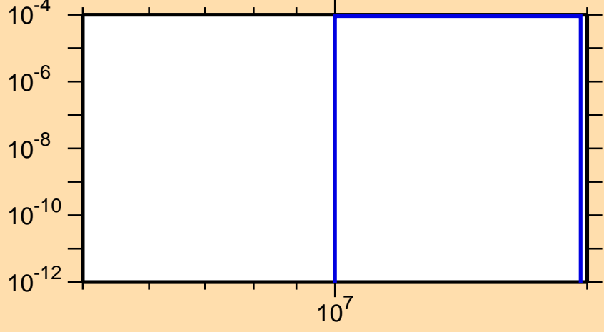
\sigma vs. E for ^{187}\text{Pb}(n,2n\alpha)
