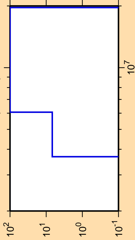
\Delta\sigma/\sigma vs. E for ^{187}\text{Pb}(n,\text{He3})
