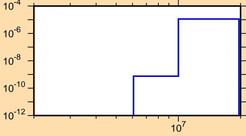
\sigma vs. E for ^{187}\text{Pb}(n,\text{He3})
