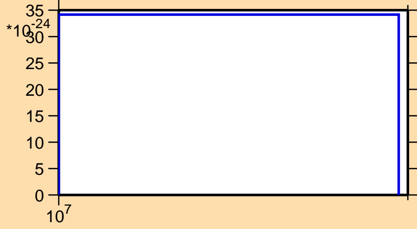
\sigma vs. E for ^{187}\text{Pb} (mt 11)
