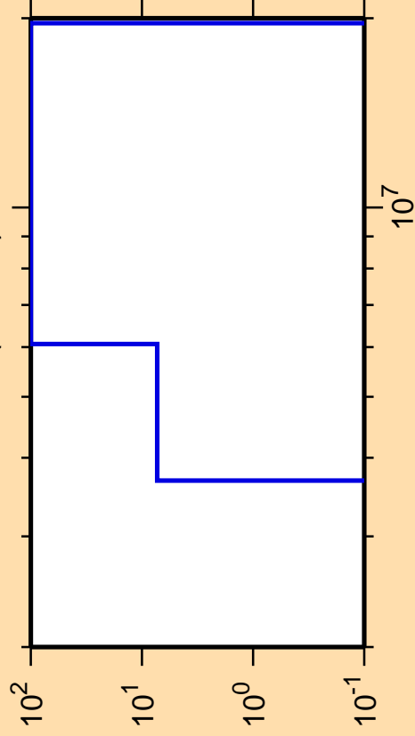
\Delta\sigma/\sigma vs. E for ^{187}\text{Pb}(\text{mt117})
