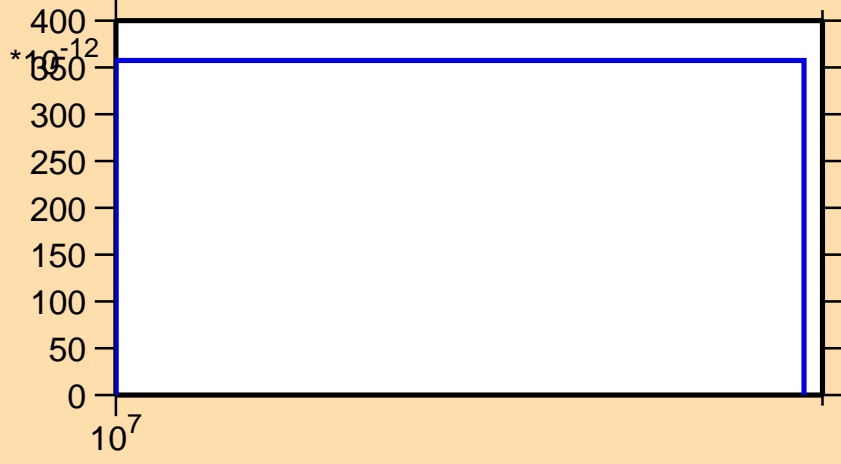
\sigma vs. E for ^{187}\text{Pb} (mt 34)
