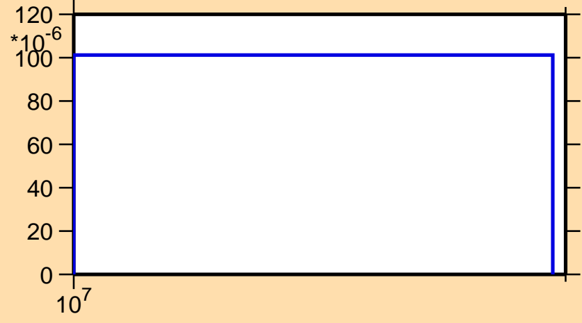
\sigma vs. E for ^{187}\text{Pb}(n,2np)
