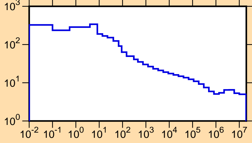
\sigma vs. E for ^{187}\text{Pb}(n,\text{tot.})
