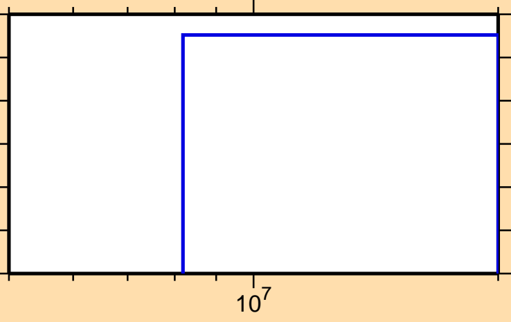
\sigma vs. E for ^{187}\text{Pb}(n,\text{nd})
