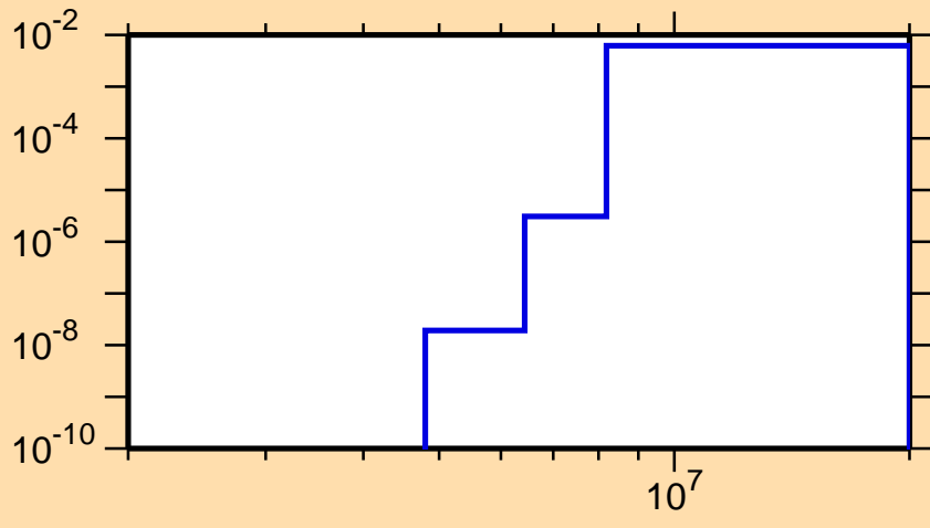
\sigma vs. E for ^{187}\text{Pb}(n,d)
