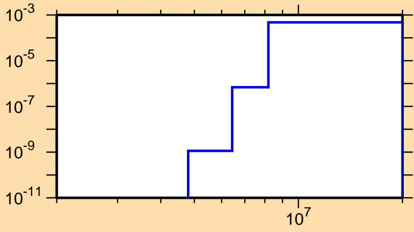
\sigma vs. E for ^{187}\text{Pb}(\text{mt } 45)
