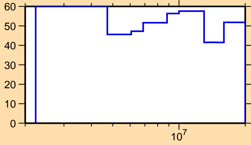
\Delta\sigma/\sigma vs. E for ^{188}\text{Pb}(n,n\text{nonel.})
