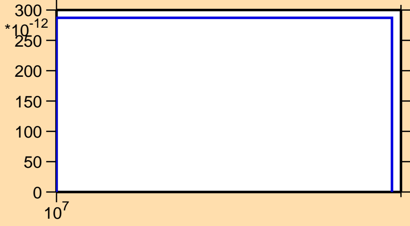
\sigma vs. E for ^{188}\text{Pb}(n,3n)
