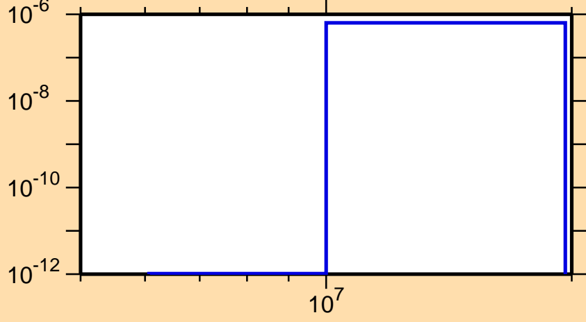
\sigma vs. E for ^{188}\text{Pb}(\text{mt } 45)
