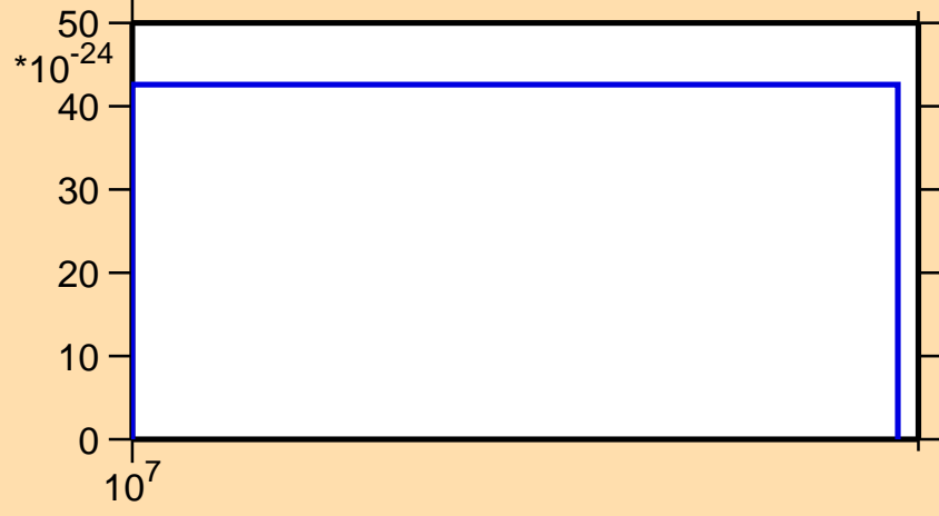
\sigma vs. E for ^{188}\text{Pb} (mt 11)
