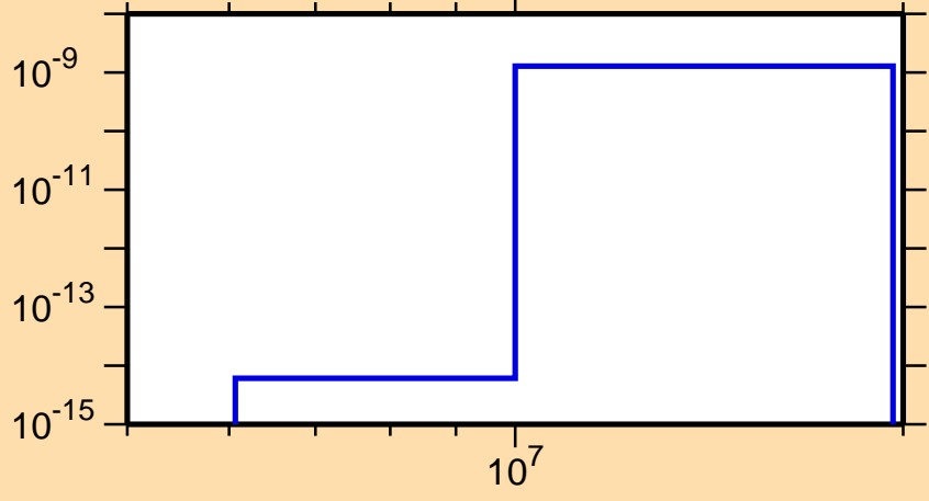
\sigma vs. E for ^{188}\text{Pb}(\text{mt117})
