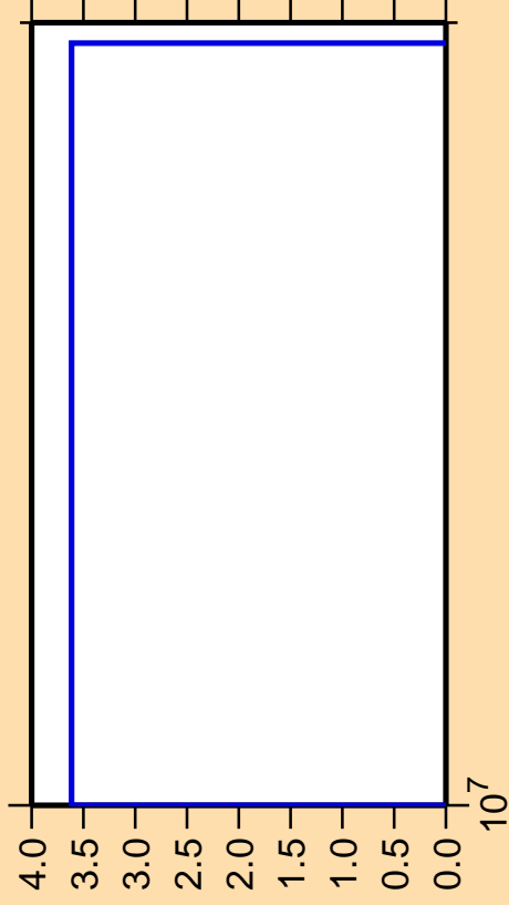
\Delta\sigma/\sigma vs. E for ^{188}\text{Pb} (mt 34)
