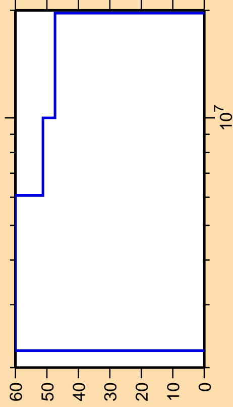
\Delta\sigma/\sigma vs. E for ^{188}\text{Pb}(n,\gamma)
