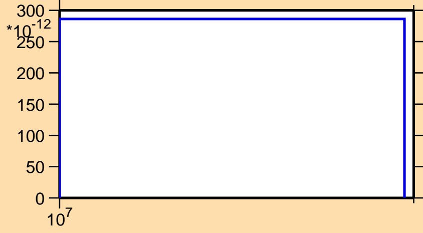
\sigma vs. E for ^{188}\text{Pb}(n,\text{nd})
