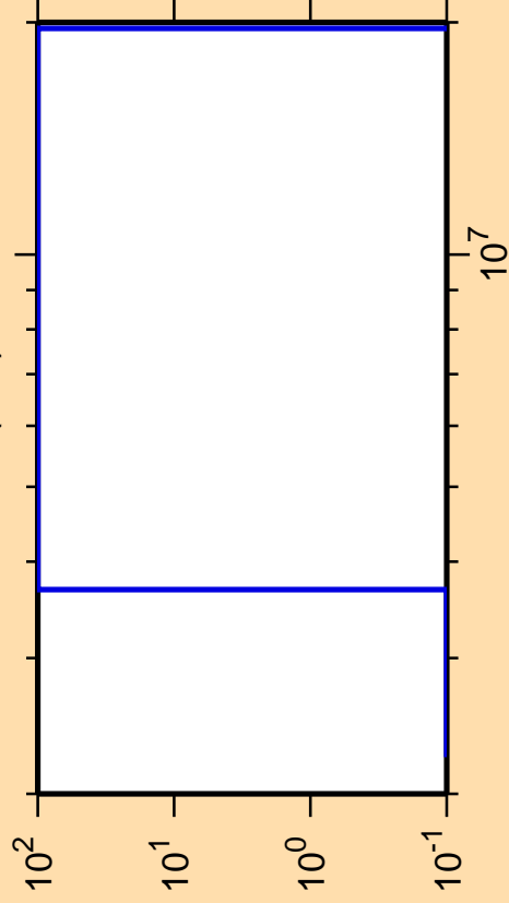
\Delta\sigma/\sigma vs. E for ^{188}\text{Pb}(n,d)
