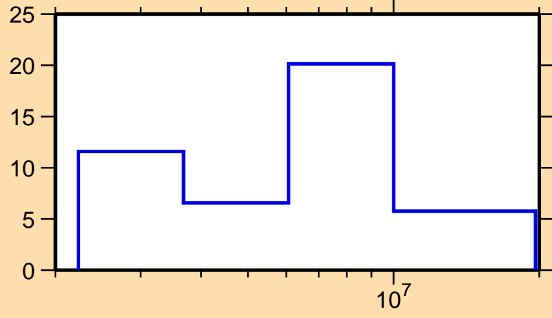
\Delta\sigma/\sigma vs. E for ^{188}\text{Pb}(n,\text{tot.})
