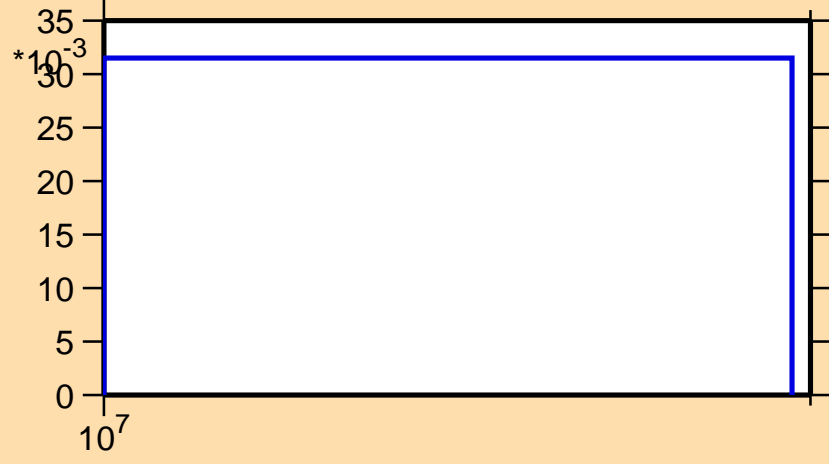
\sigma vs. E for ^{188}\text{Pb}(n,2n)
