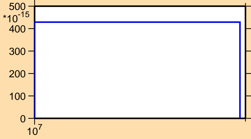
\sigma vs. E for ^{188}\text{Pb} (mt 34)
