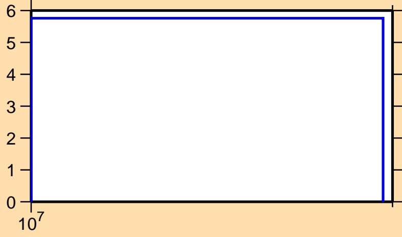
\Delta\sigma/\sigma vs. E for ^{188}\text{Pb}(n,\text{tot.})
