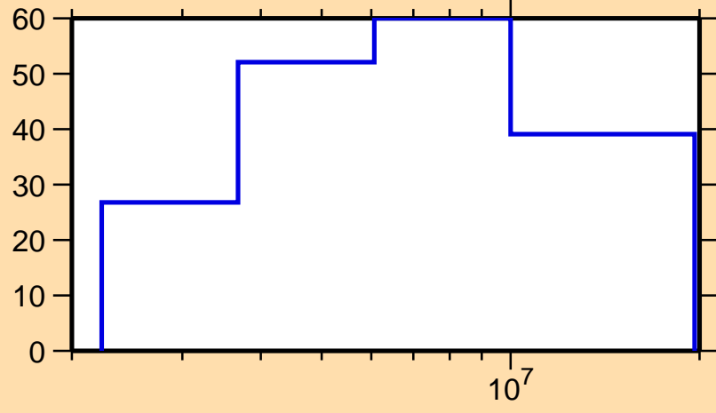
\Delta\sigma/\sigma vs. E for ^{188}\text{Pb}(n,\text{el.})
