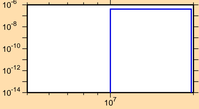
\sigma vs. E for ^{188}\text{Pb}(n,2n\alpha)
