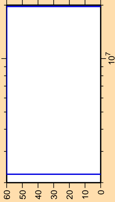
\Delta\sigma/\sigma vs. E for ^{188}\text{Pb}(n,n\text{cont.})
