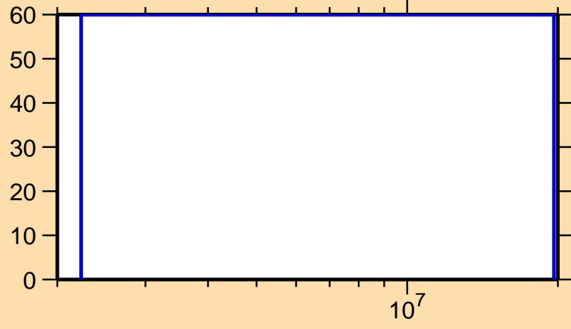
\Delta\sigma/\sigma vs. E for ^{188}\text{Pb}(n,ncont.)
