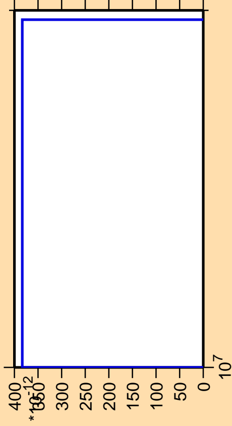
\Delta\sigma/\sigma vs. E for ^{188}\text{Pb} (mt 11)
