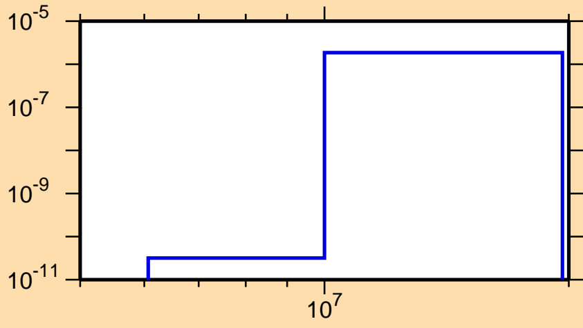
\sigma vs. E for ^{188}\text{Pb}(n,\text{He3})
