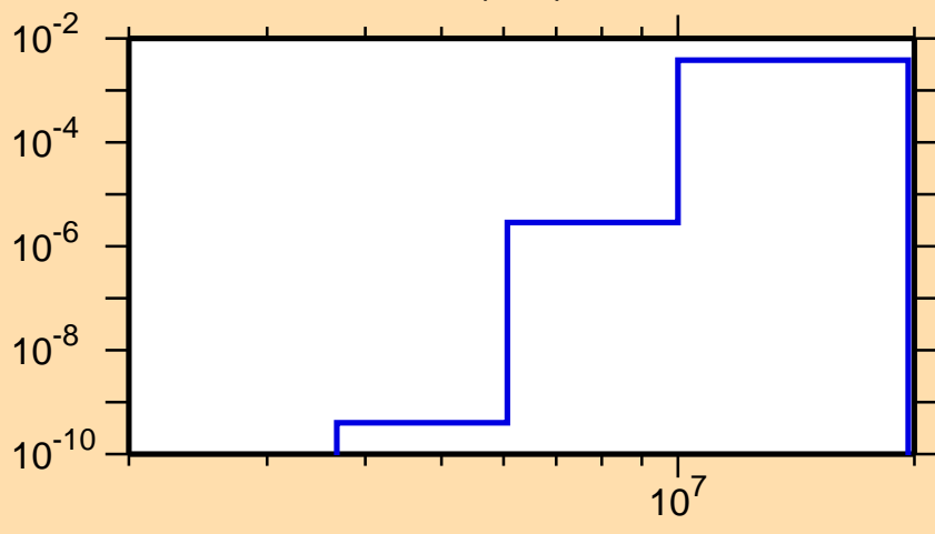
\sigma vs. E for ^{188}\text{Pb}(n,d)
