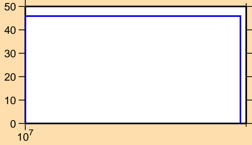
\Delta\sigma/\sigma vs. E for ^{188}\text{Pb}(n,\text{nonel.})
