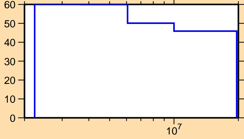
\Delta\sigma/\sigma vs. E for ^{188}\text{Pb}(n,n\text{onel.})
