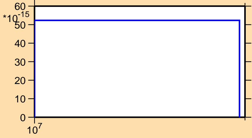
\sigma vs. E for ^{188}\text{Pb}(n,nt)
