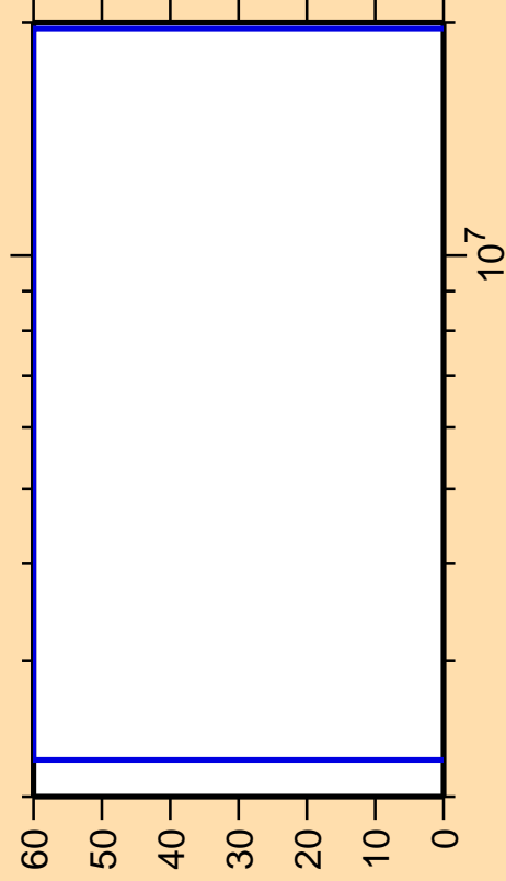
\Delta\sigma/\sigma vs. E for ^{188}\text{Pb}(n,p)
