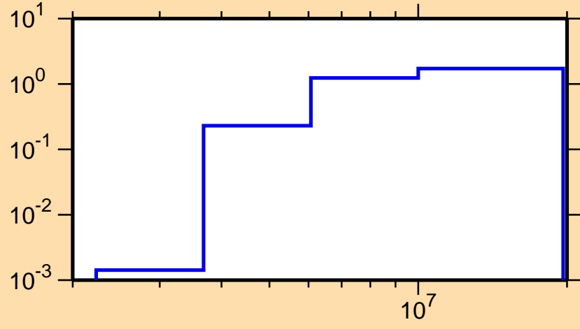
\sigma vs. E for ^{188}\text{Pb}(n,n\text{cont.})
