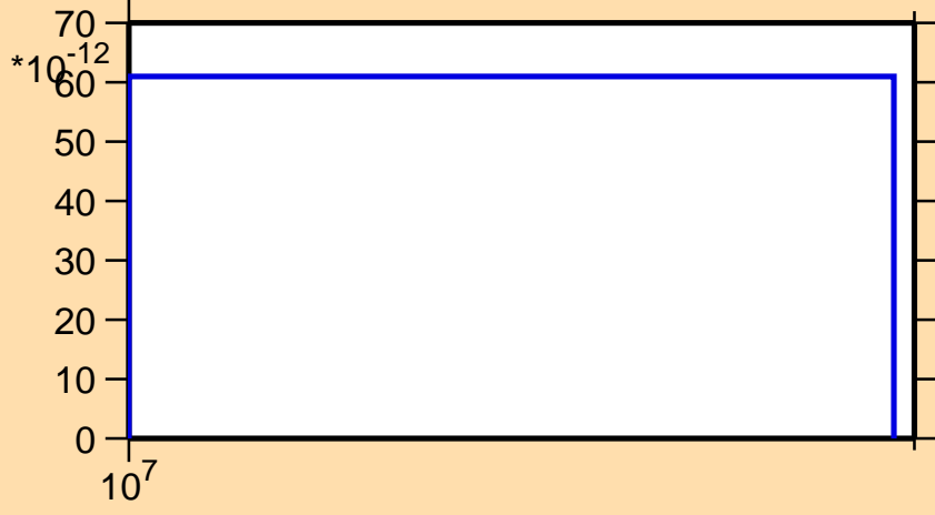
\sigma vs. E for ^{188}\text{Pb}(n,\text{pt})
