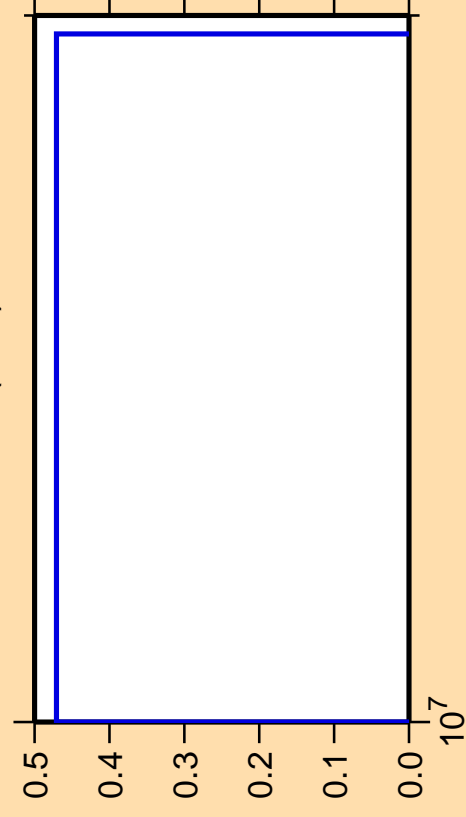
\Delta\sigma/\sigma vs. E for ^{188}\text{Pb}(n,nt)
