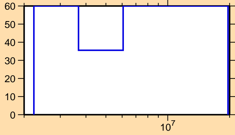
\Delta\sigma/\sigma vs. E for ^{188}\text{Pb}(n,\text{inel.})
