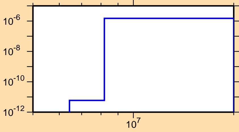
\sigma vs. E for ^{188}\text{Pb}(n,\text{He3})
