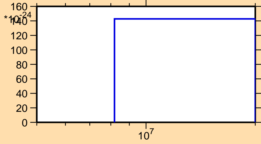
\sigma vs. E for ^{188}\text{Pb}(\text{mt } 11)
