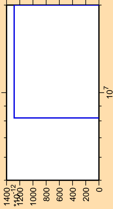
\Delta\sigma/\sigma vs. E for ^{188}\text{Pb}(\text{mt } 11)
