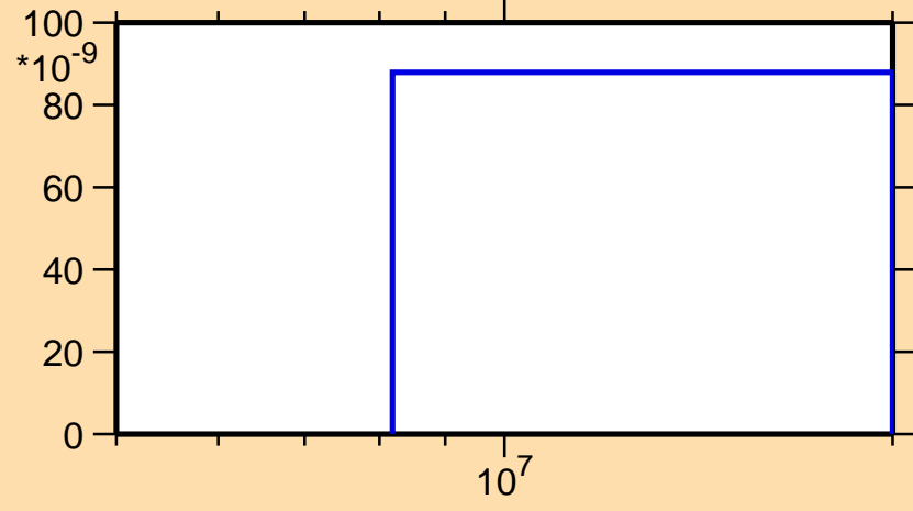
\sigma vs. E for ^{188}\text{Pb}(n,\text{pd})
