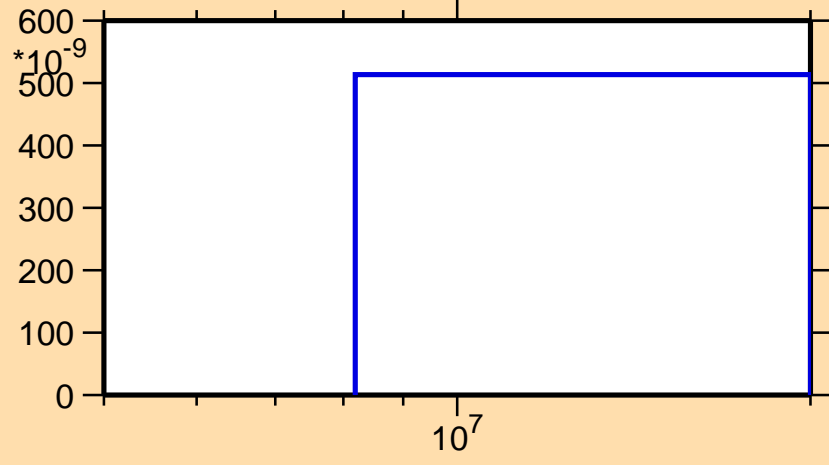
\sigma vs. E for ^{188}\text{Pb}(\text{mt } 45)
