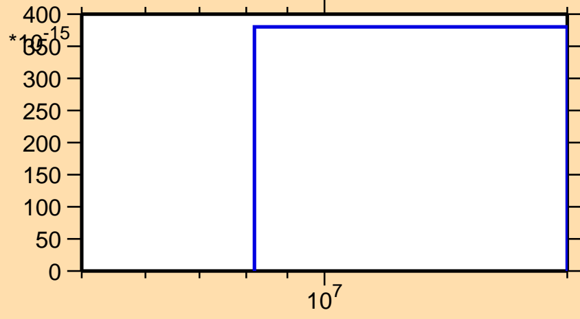
\sigma vs. E for ^{188}\text{Pb}(\text{mt } 34)
