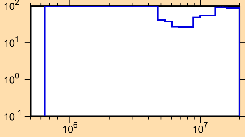
\Delta\sigma/\sigma vs. E for ^{189}\text{Pb}(n,ncont.)
