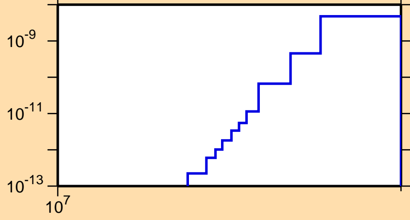
\sigma vs. E for ^{189}\text{Pb}(\text{mt } 34)
