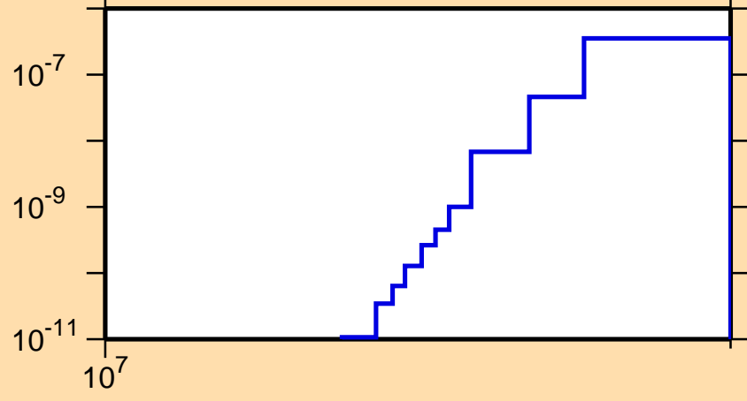
\sigma vs. E for ^{189}\text{Pb}(n,\text{pt})
